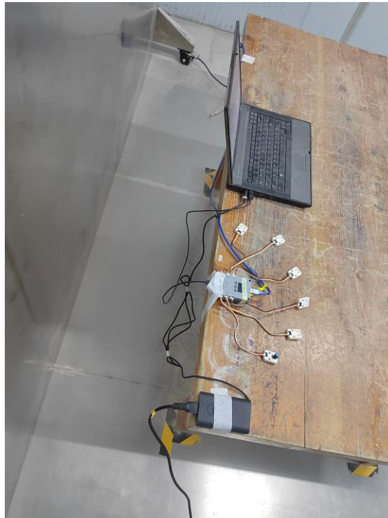
Conducted Emissions Side View
