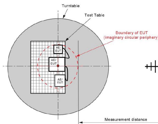
Figure C.1 – Measurement distance
