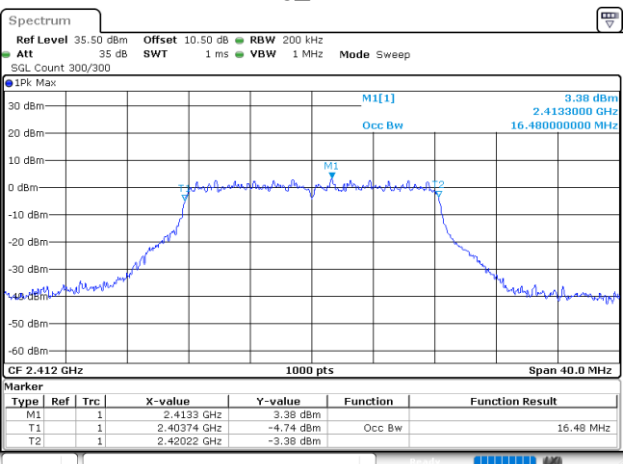
802.11g_2412MHz
