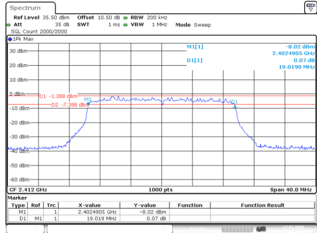
802.11ax20_2412MHz_RU_Full
