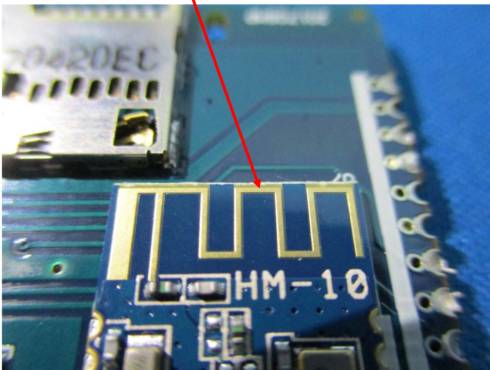
PCB Antenna – Location View
