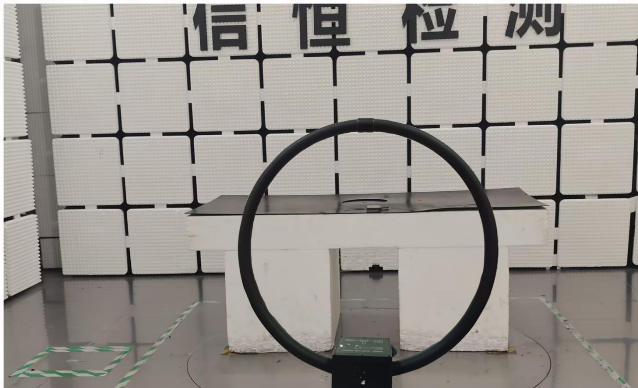
Emissions in Non-restricted Frequency Bands(9KHz - 30MHz)
