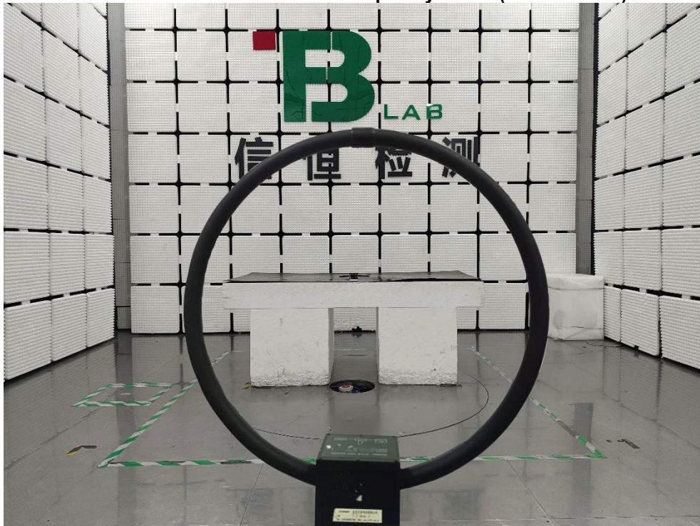
Emissions in Non-restricted Frequency Bands(9kHz-30 MHz)
