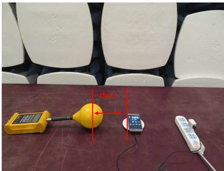
Test Position A-Exposure photo from side edge surface-Left
