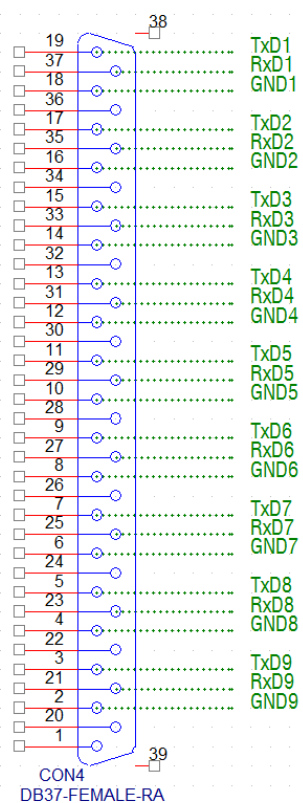
B. Serial Connector Pin map.
