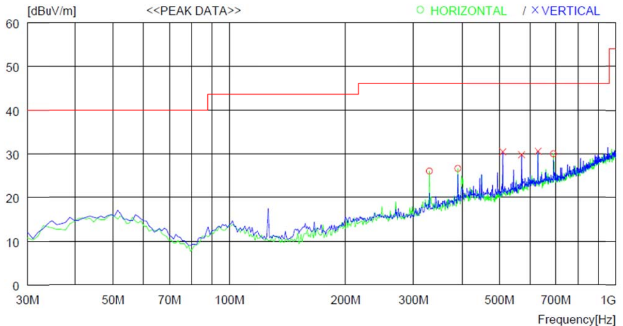
Graphical Test Data – Below 1 GHz(802.11g, High Channel)
