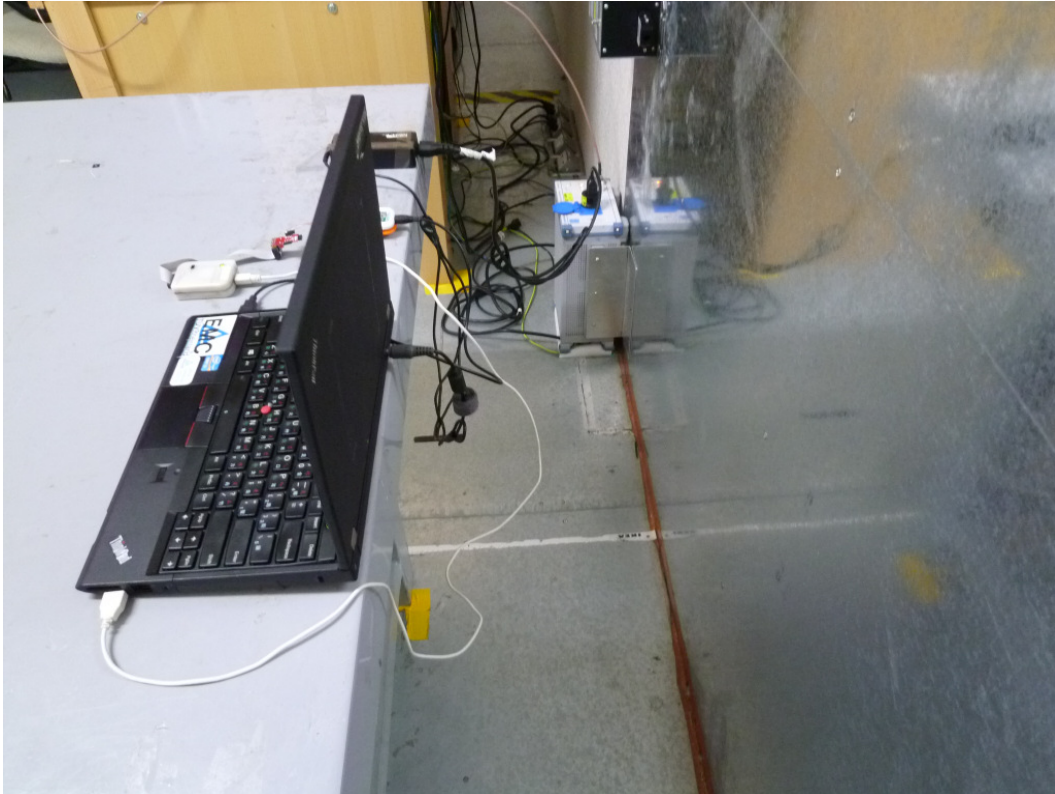
Photograph 7: Set-up for Mains (Back View)
