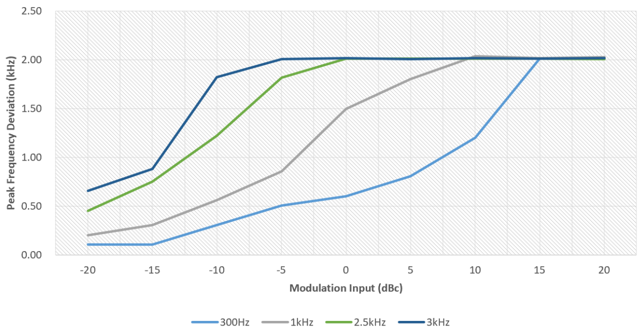
Modulation Characteristics
