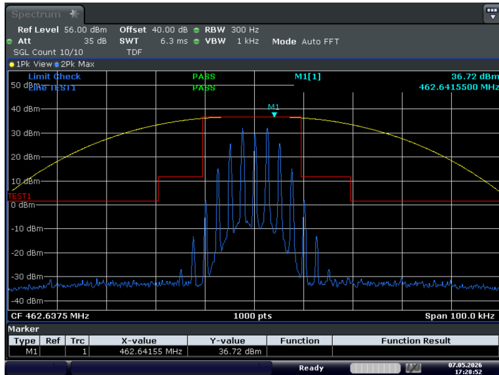
Test_Graph_GMRS_5W_462.6375_25k_Mask_D
