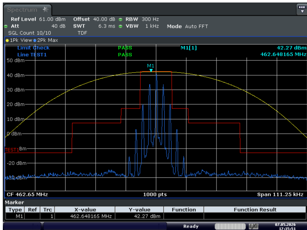
Test_Graph_GMRS_15W_462.65_12.5k_Mask_D
