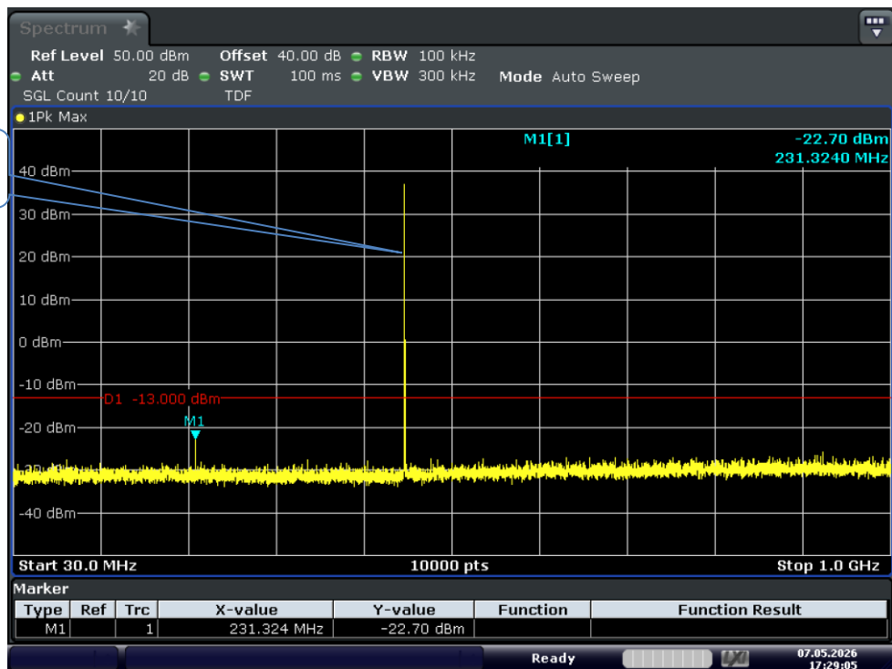
Test_Graph_GMRS_5W_462.6375_25k_TX_0.03G-1G
