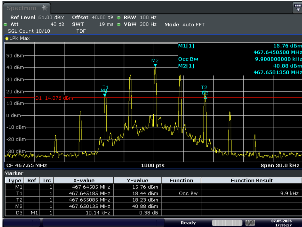
Test_Graph_GMRS_15W_467.65_12.5k_OBW
