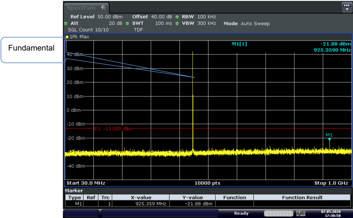
Test_Graph_GMRS_15W_462.65_25k_TX_0.03G-1G
