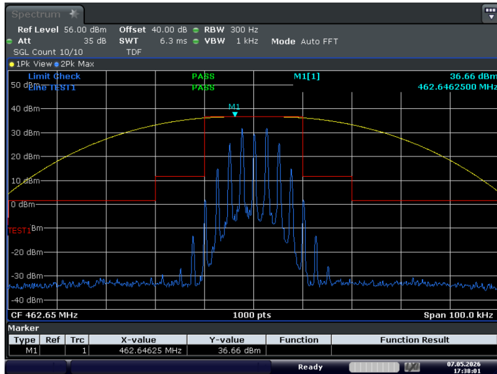
Test_Graph_GMRS_5W_462.65_25k_Mask_D
