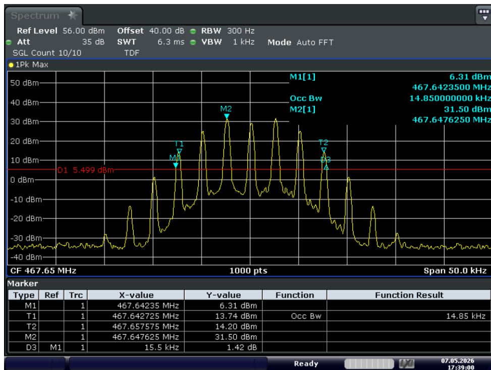
Test_Graph_GMRS_5W_467.65_12.5k_OBW
