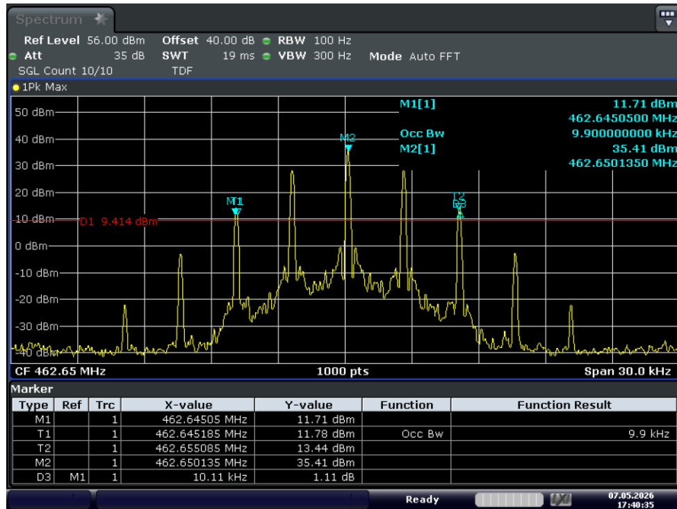
Test_Graph_GMRS_5W_462.65_12.5k_OBW
