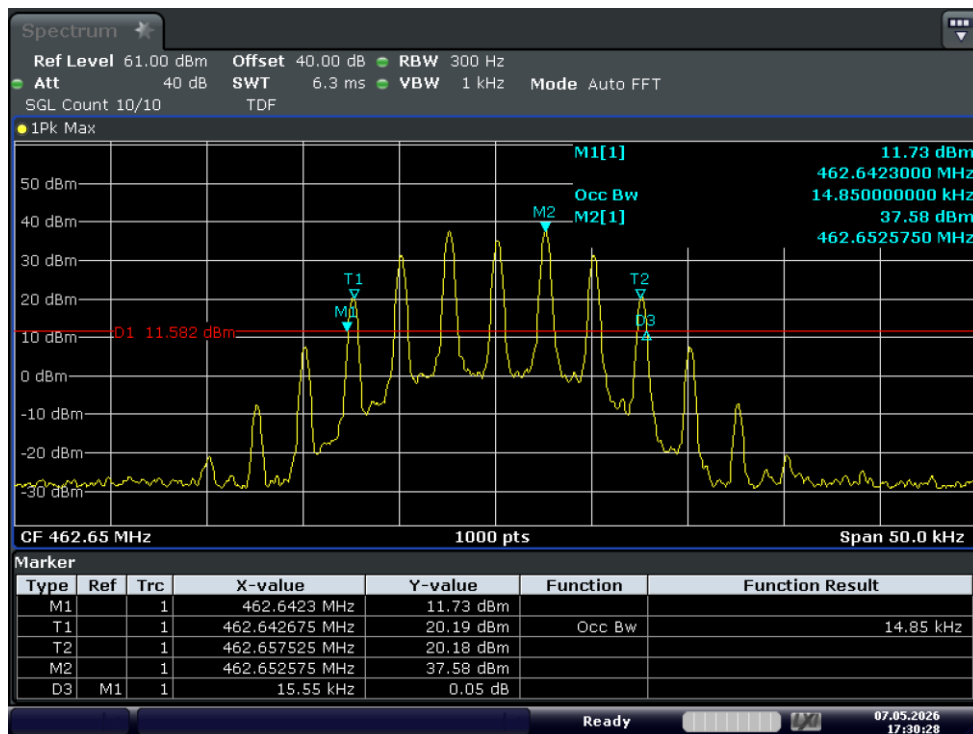
Test_Graph_GMRS_15W_462.65_12.5k_OBW
