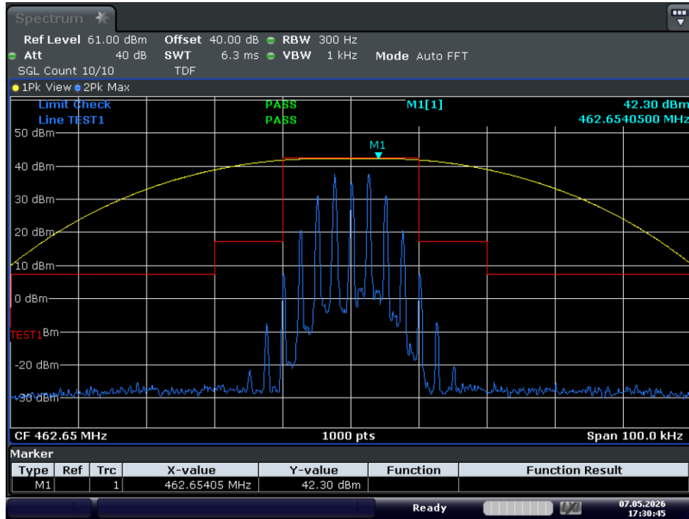
Test_Graph_GMRS_15W_462.65_25k_Mask_D
