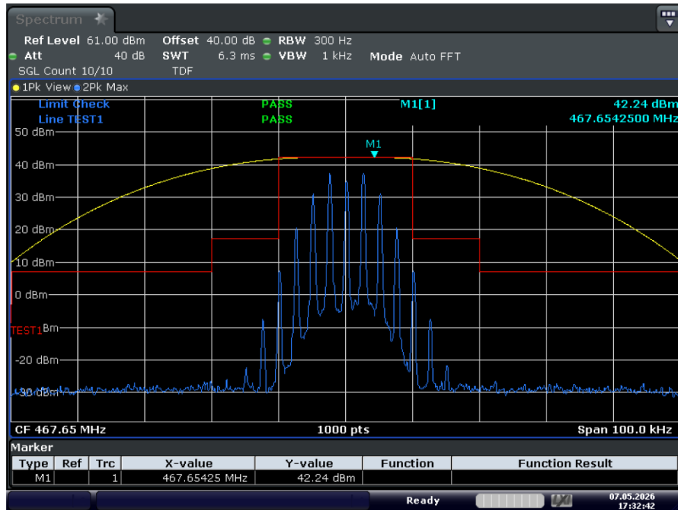
Test_Graph_GMRS_15W_467.65_25k_Mask_D
