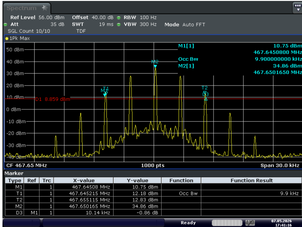
Test_Graph_GMRS_5W_467.65_12.5k_OBW
