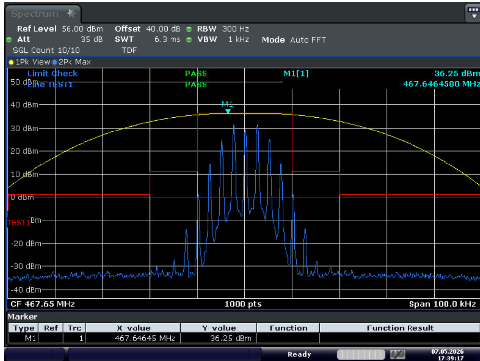
Test_Graph_GMRS_5W_467.65_25k_Mask_D
