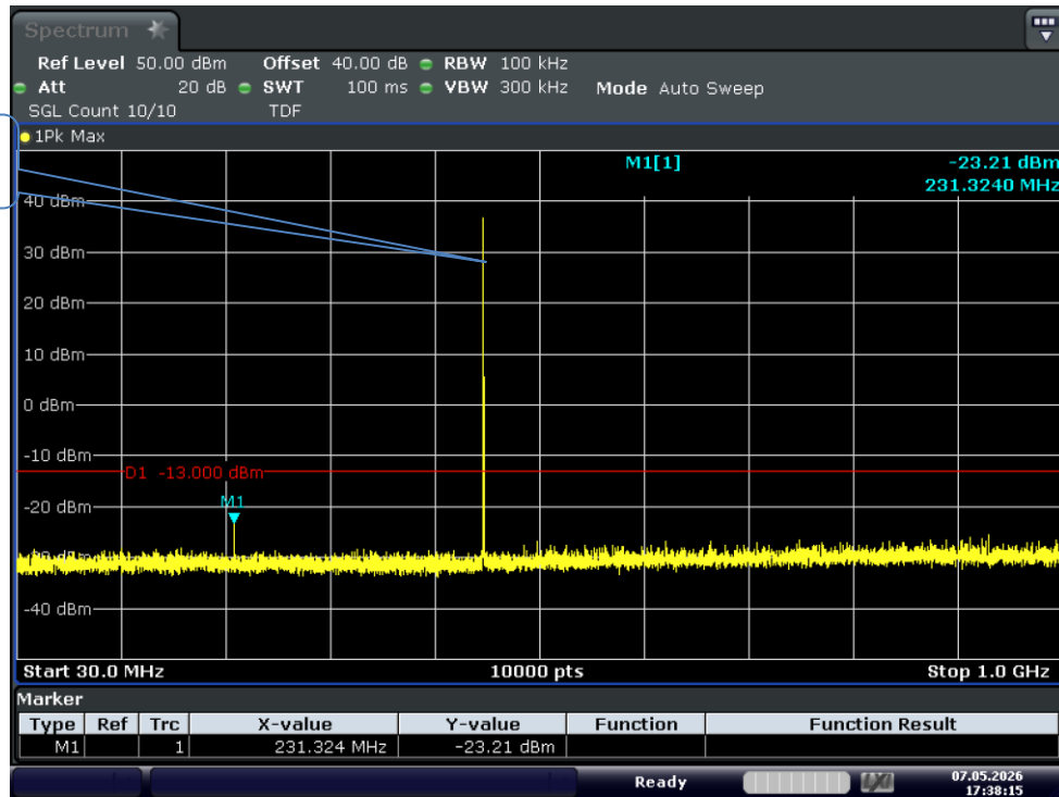
Test_Graph_GMRS_5W_462.65_25k_TX_0.03G-1G
