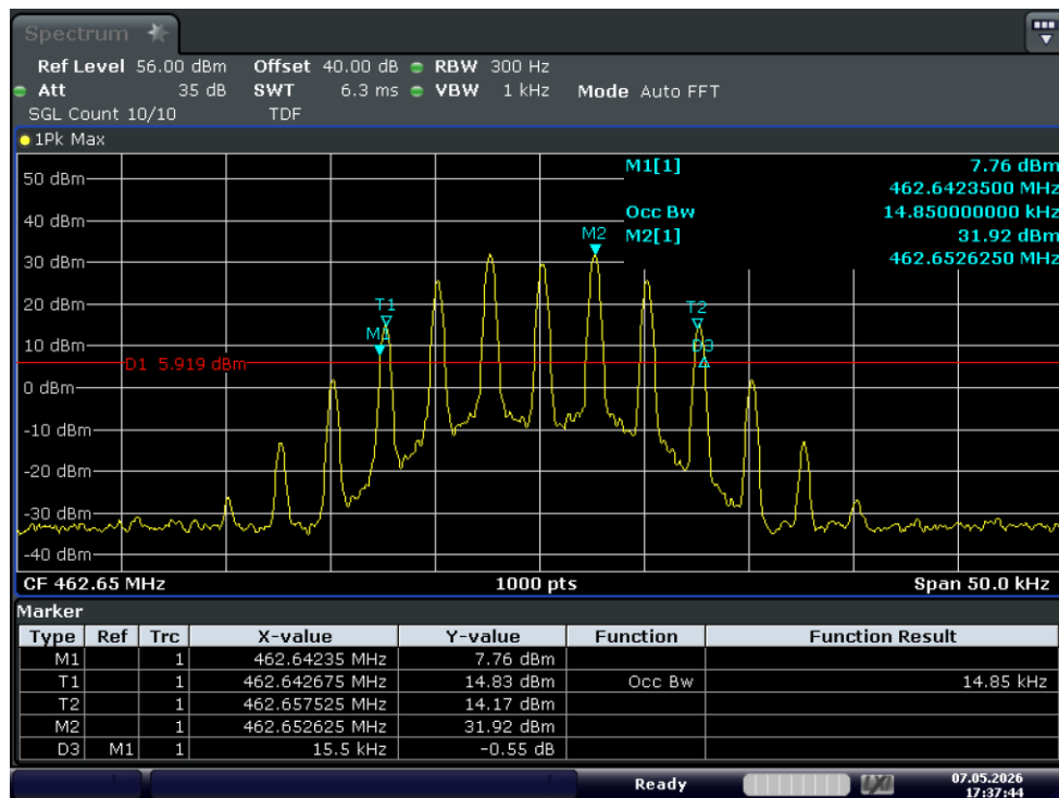
Test_Graph_GMRS_5W_462.65_12.5k_OBW
