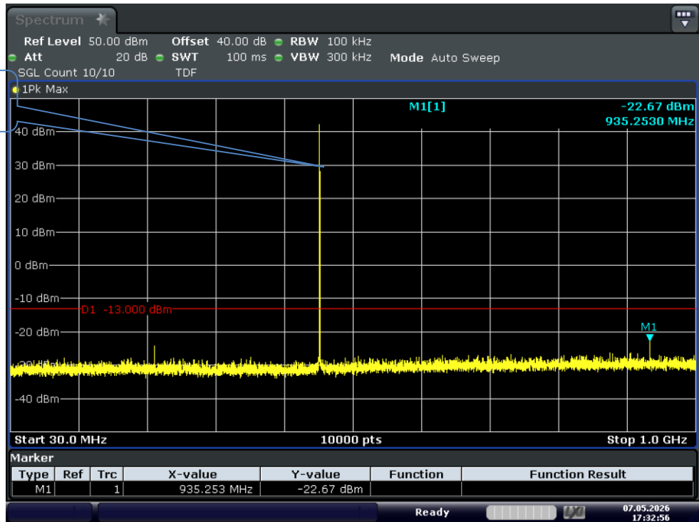
Test_Graph_GMRS_15W_467.65_25k_TX_0.03G-1G
