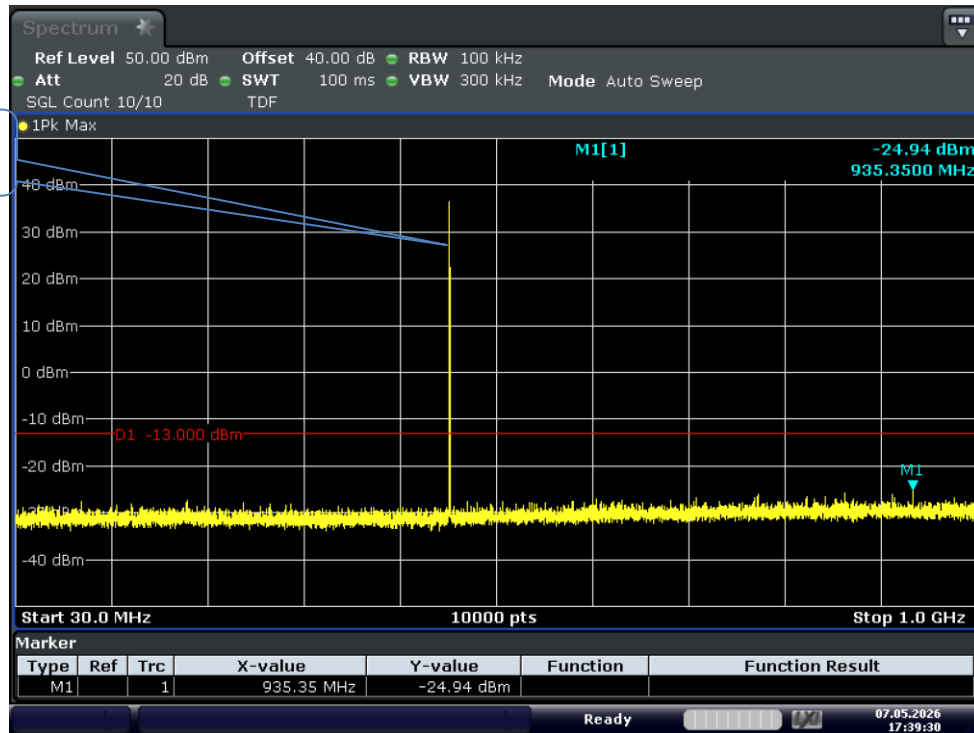
Test_Graph_GMRS_5W_467.65_25k_TX_0.03G-1G
