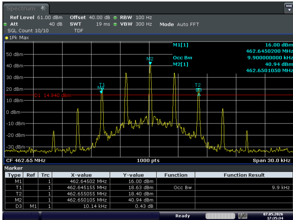
Test_Graph_GMRS_15W_462.65_12.5k_OBW
