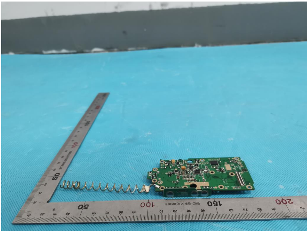
4Internal View-9 of EUT
