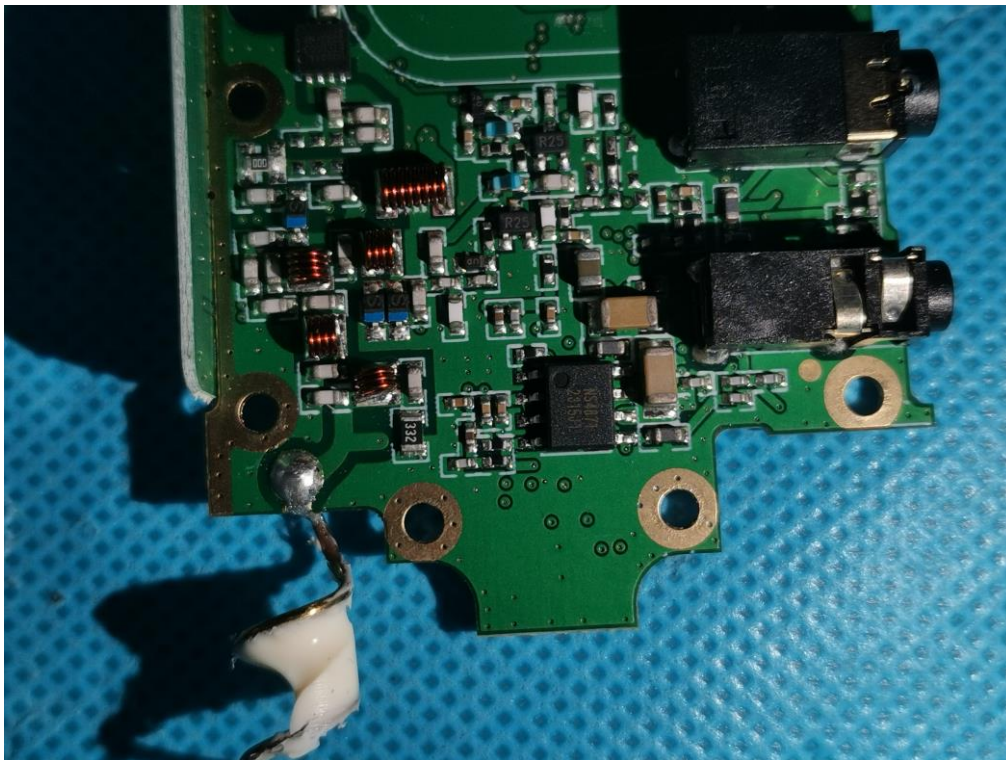
4Internal View-11 of EUT
