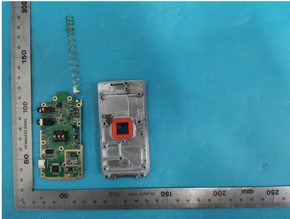
4Internal View-5 of EUT
