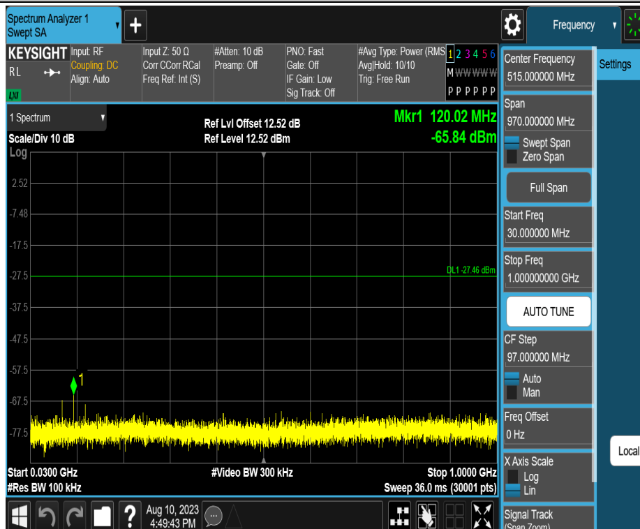
BLE_1M_Ant1_2402_30~1000
