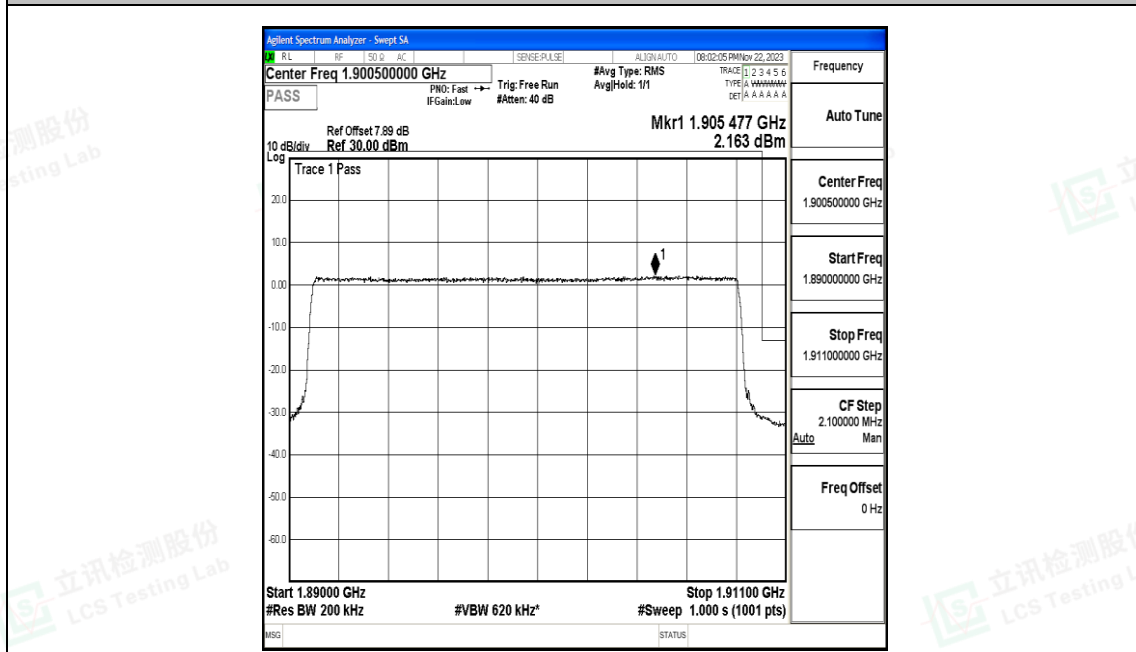
Band2_20MHz_16QAM_19100_100RB#0
