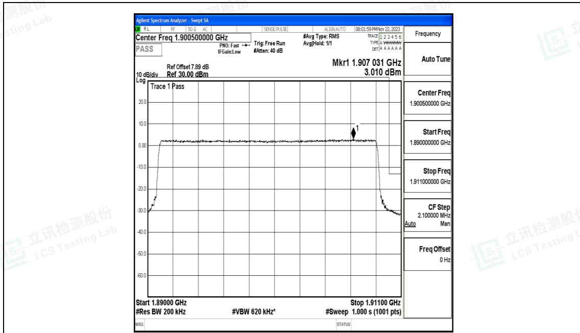
Band2_20MHz_QPSK_19100_100RB#0
