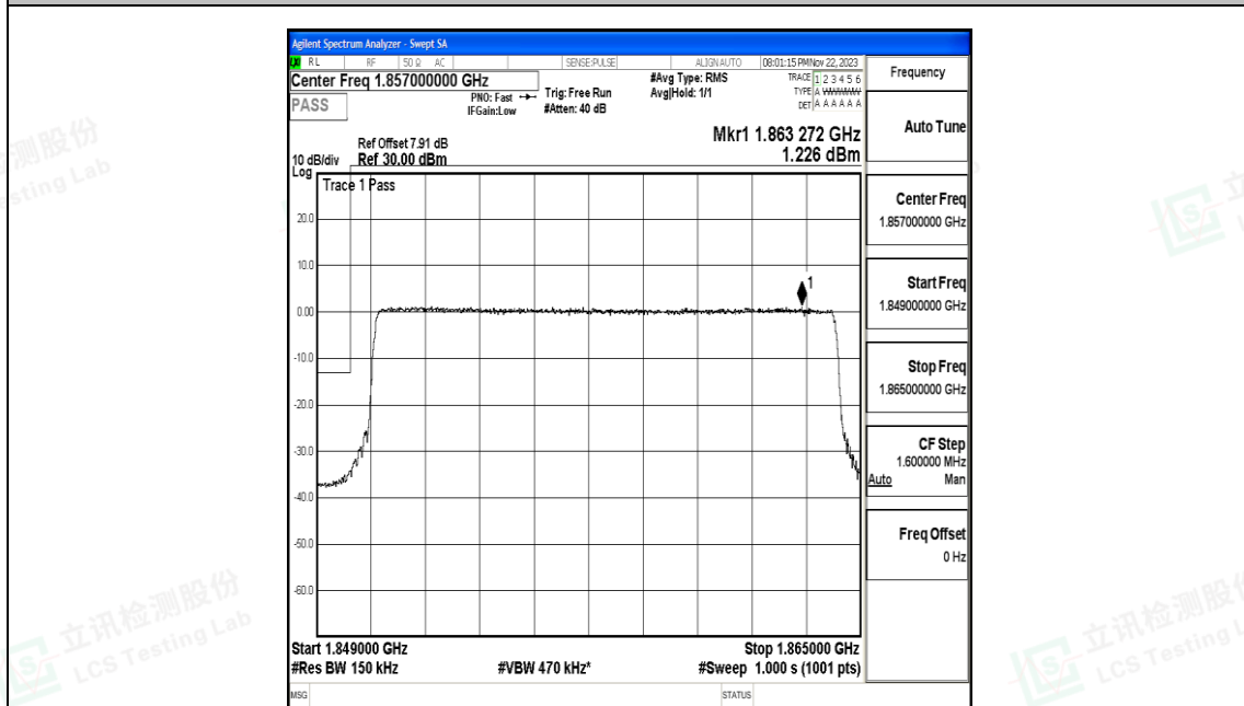
Band2_15MHz_QPSK_18675_75RB#0
