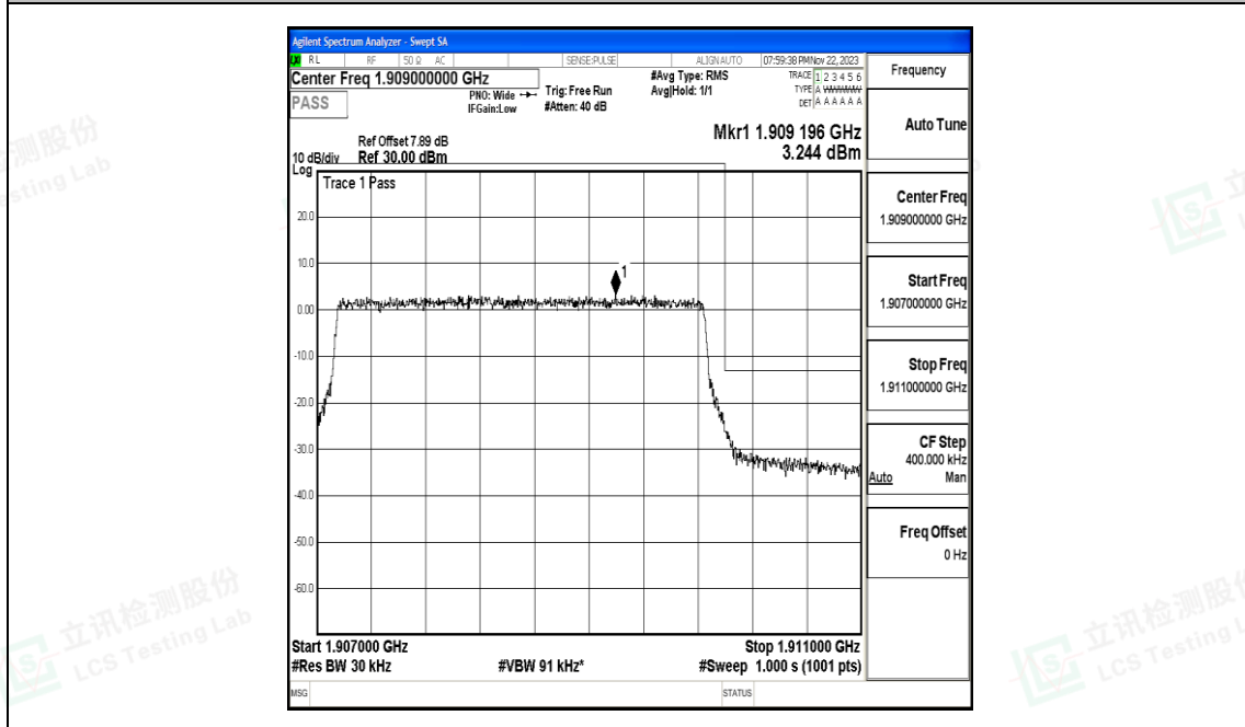
Band2_3MHz_16QAM_19185_15RB#0
