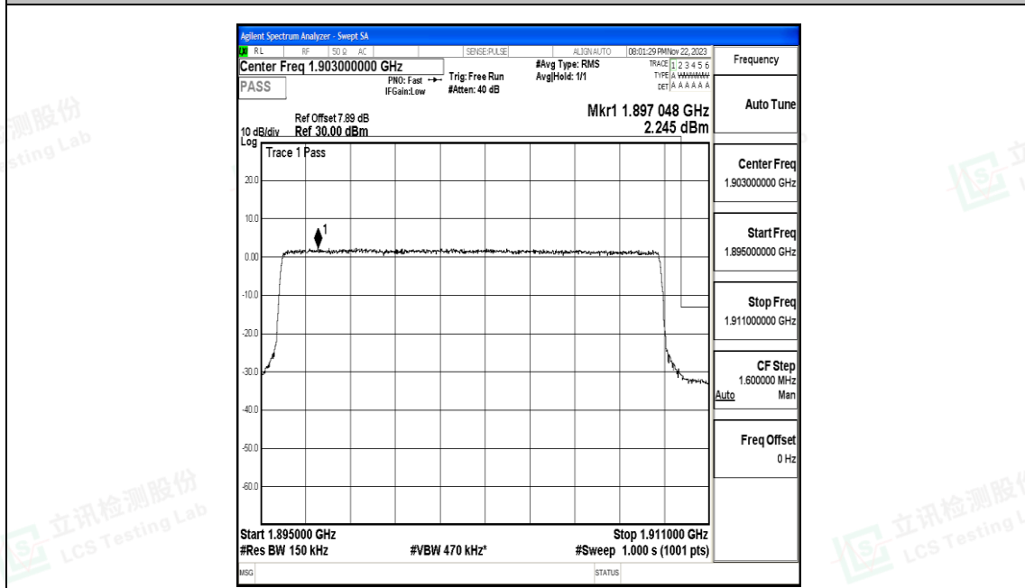
Band2_15MHz_16QAM_19125_75RB#0
