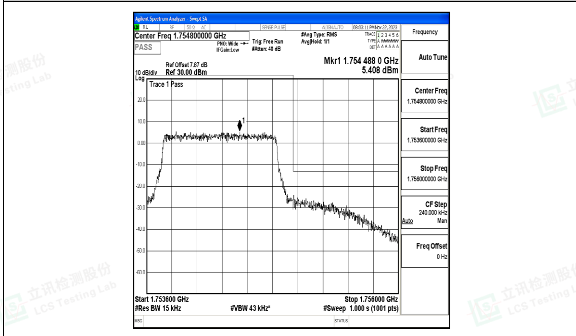
Band4_1.4MHz_16QAM_20393_6RB#0
