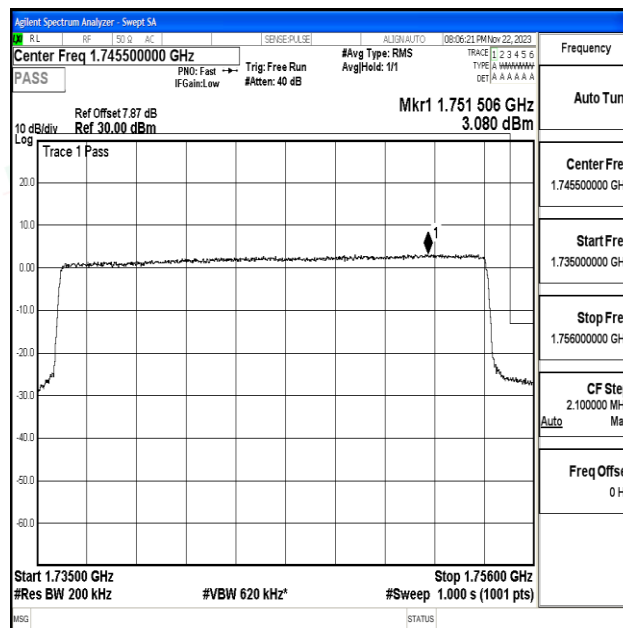
Band4_20MHz_16QAM_20300_100RB#0
