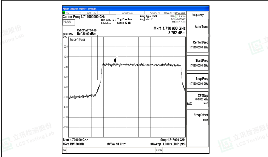
Band4_3MHz_16QAM_19965_15RB#0
