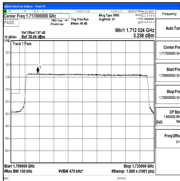
Band4_15MHz_16QAM_20025_75RB#0
