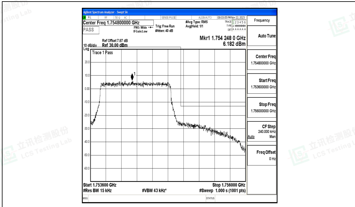
Band4_1.4MHz_QPSK_20393_6RB#0
