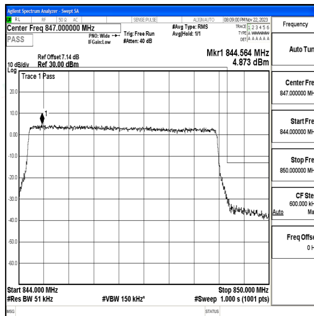
Band5_5MHz_QPSK_20625_25RB#0
