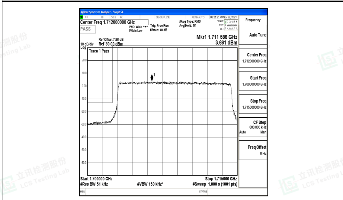
Band66_5MHz_16QAM_131997_25RB#0
