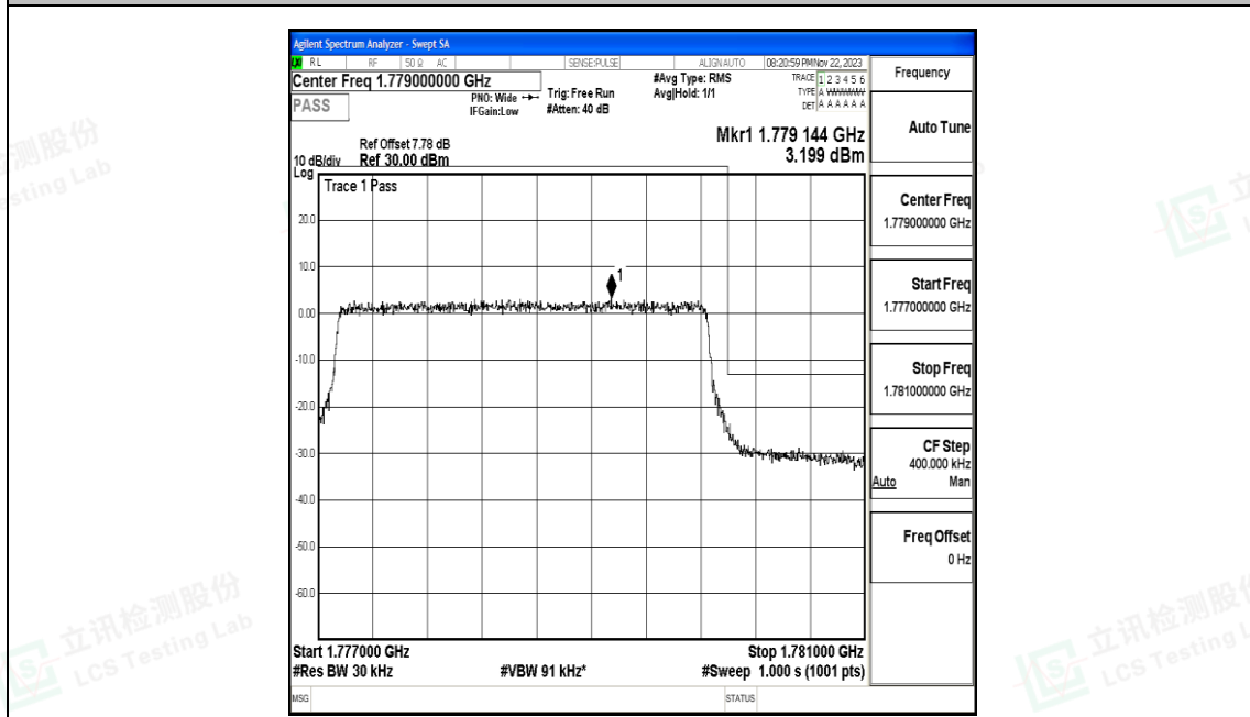
Band66_3MHz_16QAM_132657_15RB#0
