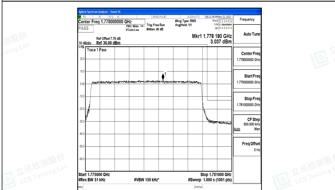
Band66_5MHz_16QAM_132647_25RB#0
