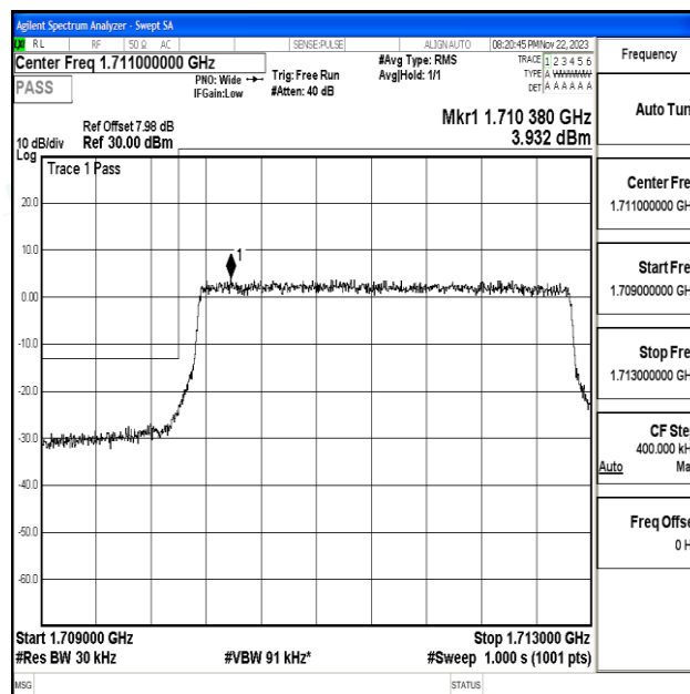
Band66_3MHz_16QAM_131987_15RB#0
