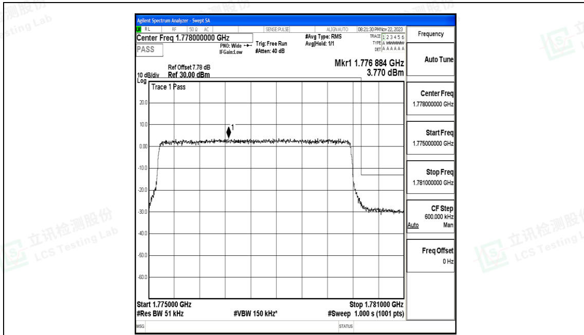
Band66_5MHz_QPSK_132647_25RB#0
