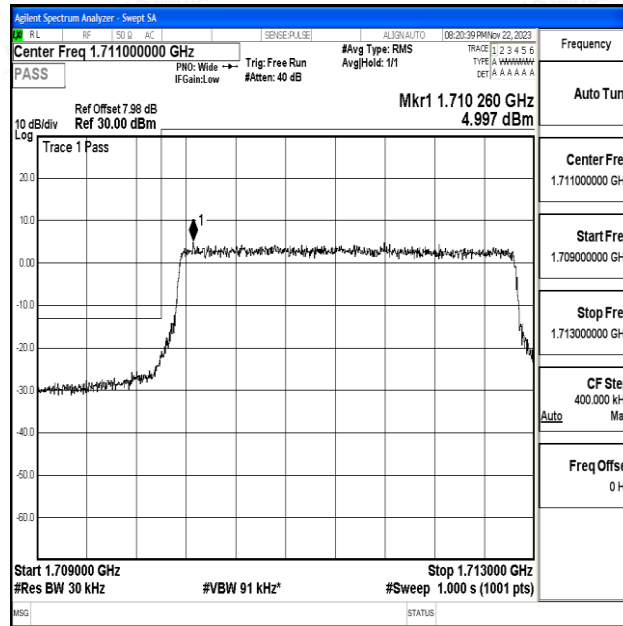
Band66_3MHz_QPSK_131987_15RB#0
