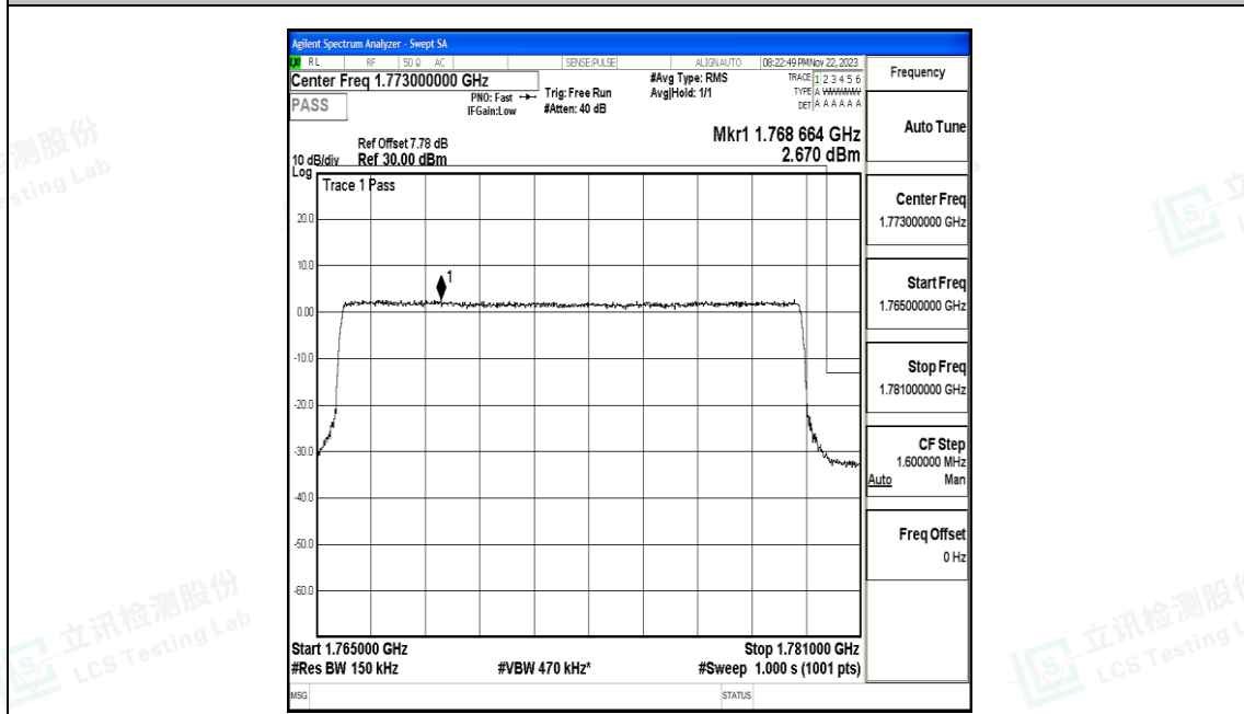
Band66_15MHz_16QAM_132597_75RB#0
