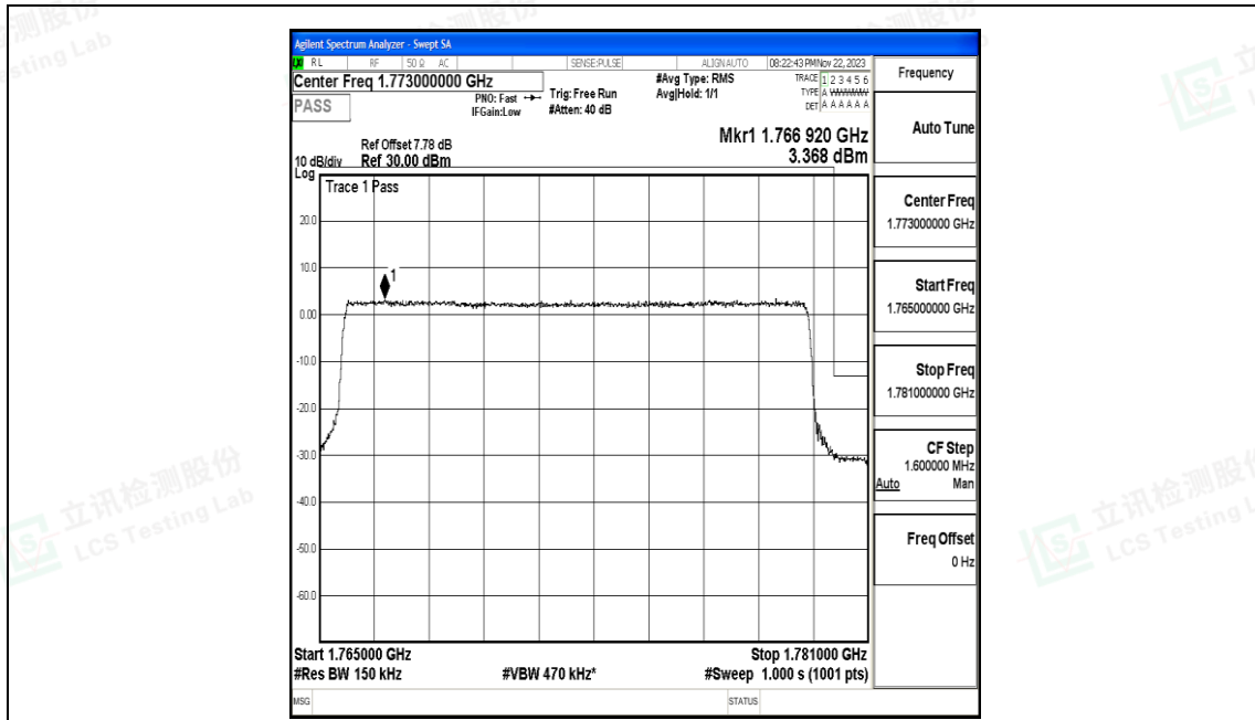
Band66_15MHz_QPSK_132597_75RB#0
