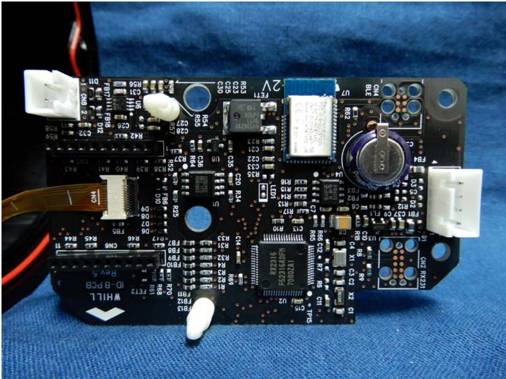
Raytac Part No. MDBT42Q-P Antenna Type. PCB Antenna
