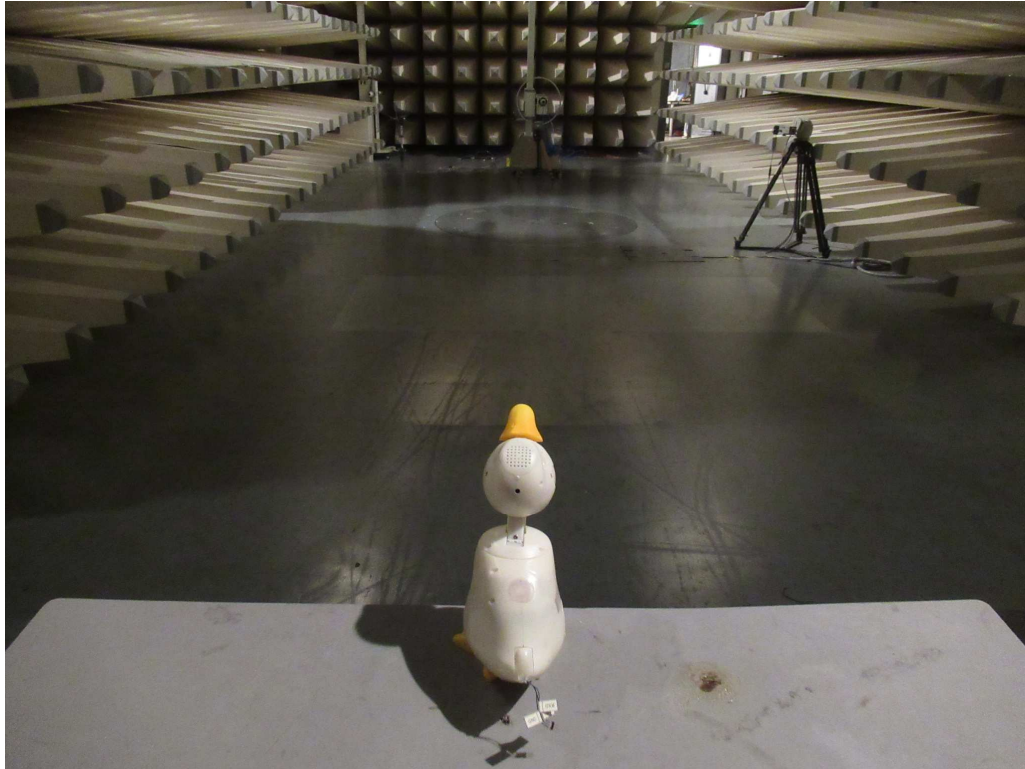
Setup for Radiated Emission (RFID)
