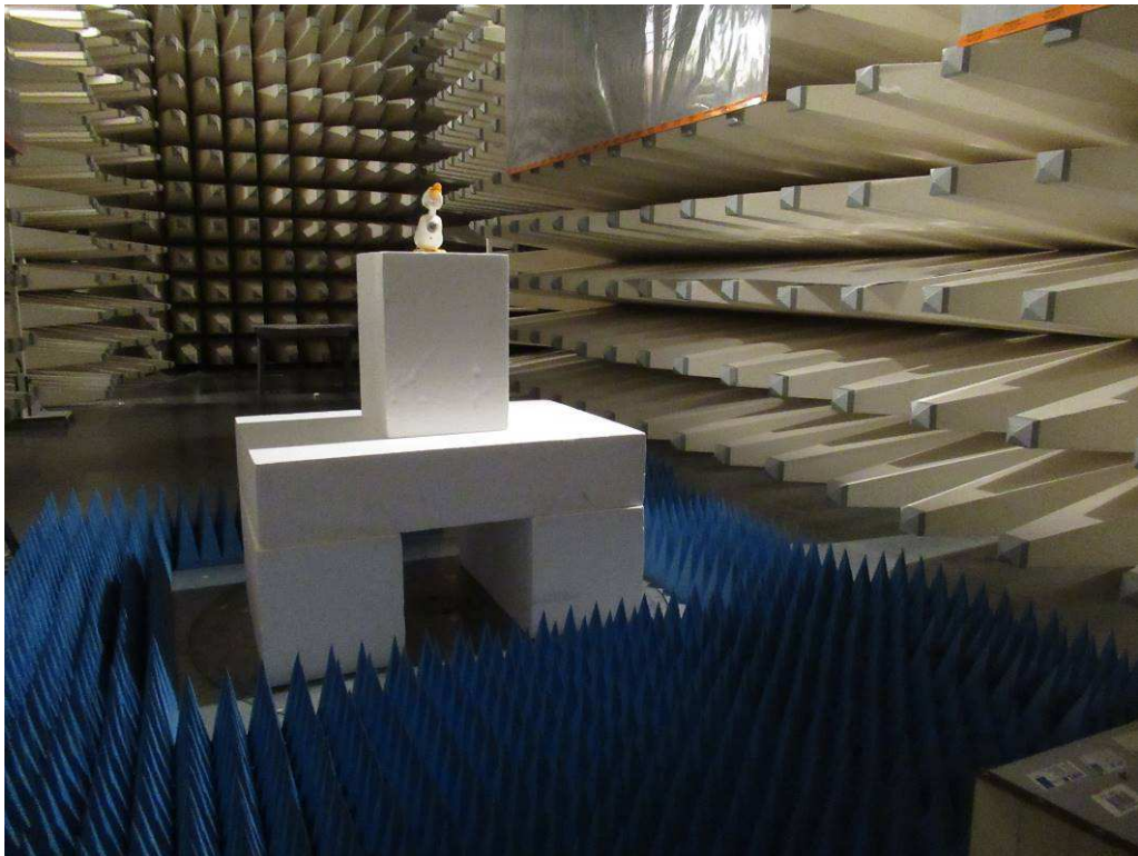
Setup for Radiated Emission (Bluetooth Low Energy)
