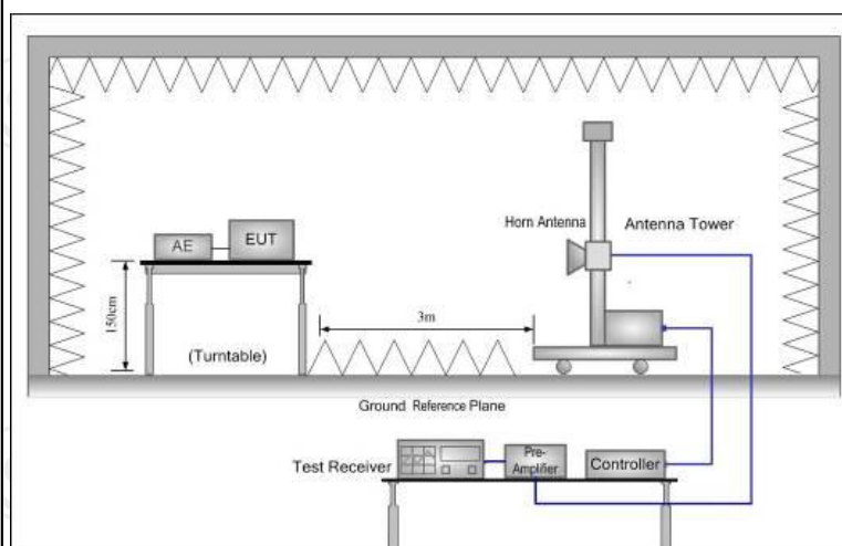
Above 1GHz
