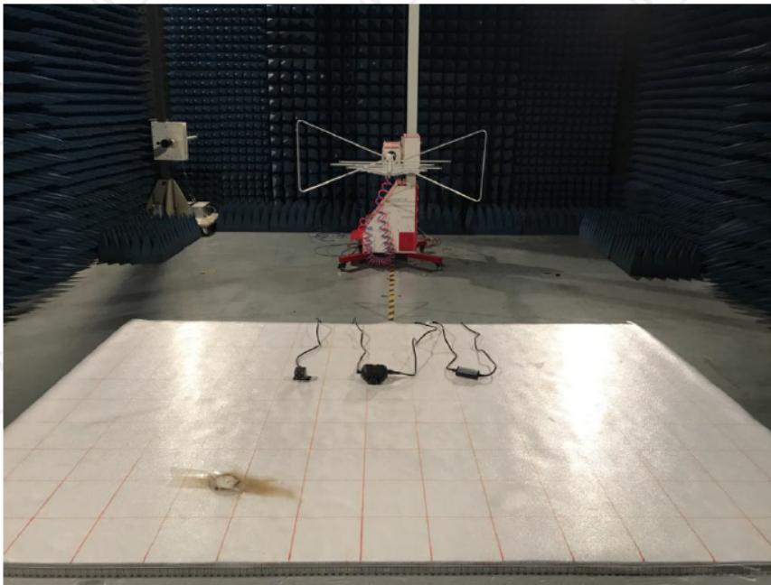
Radiated Emission
