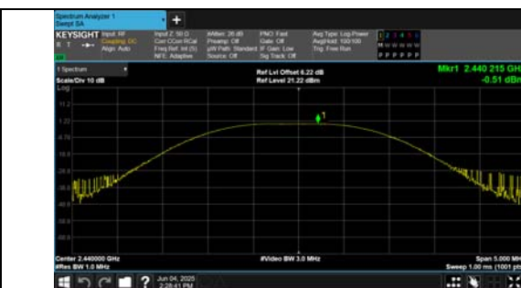
Peak Output Power BLE 1M_Channel 19
