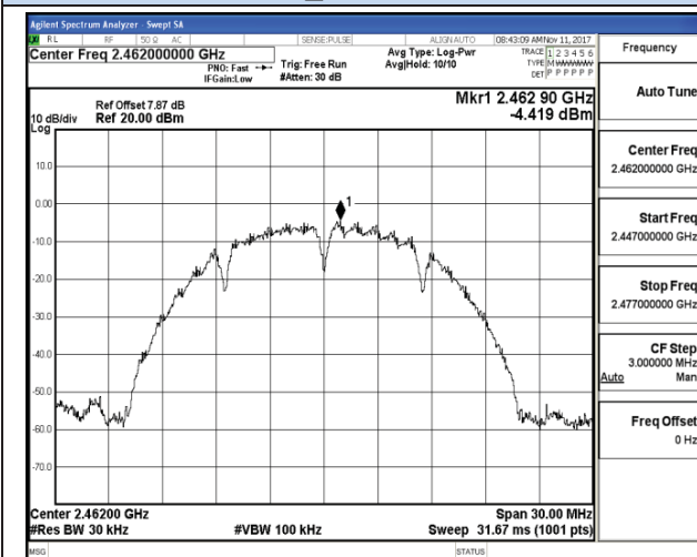
802.11b_High Channel
