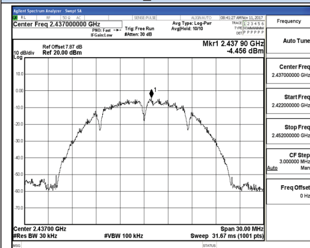
802.11b_Middle Channel
