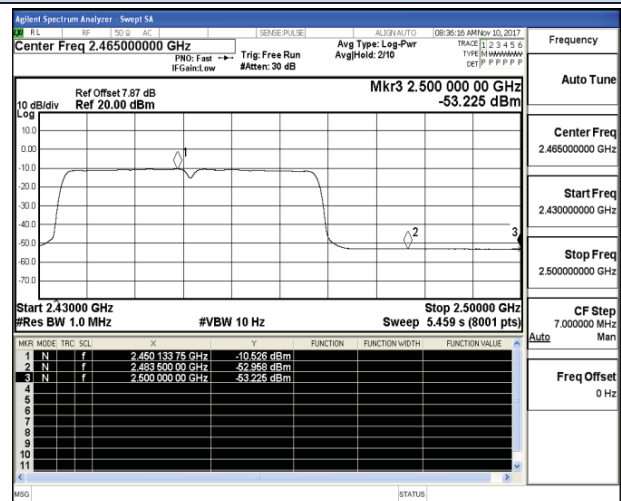
802.11n-HT40 High channel(Average)
