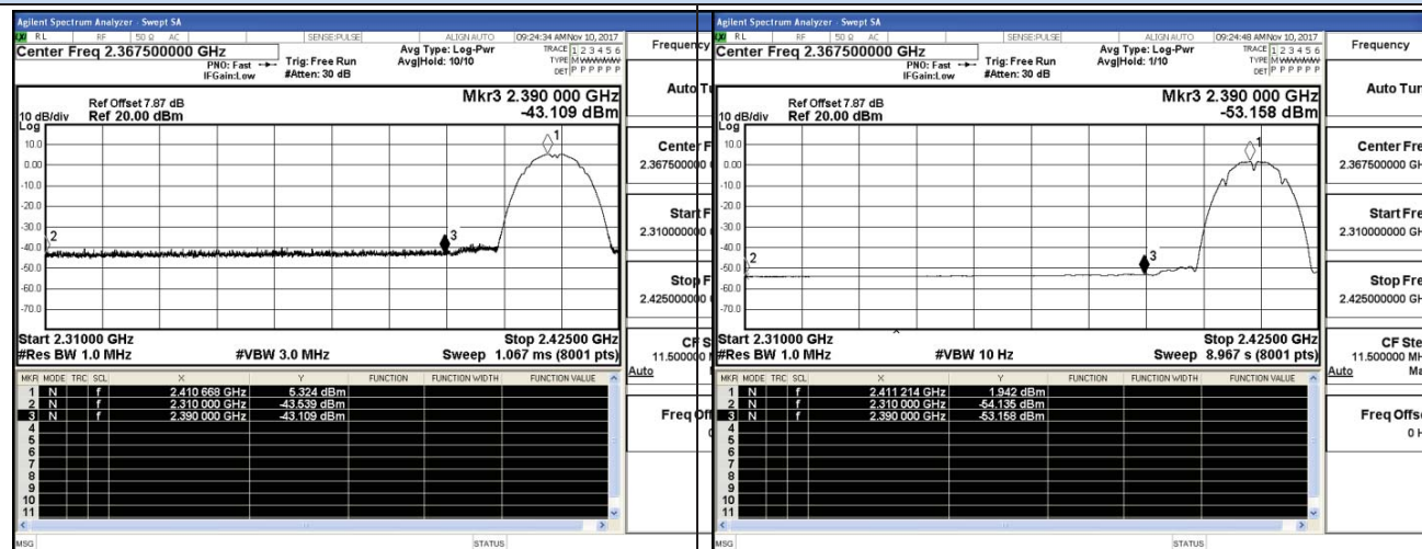
802.11b Low channel(Peak)
