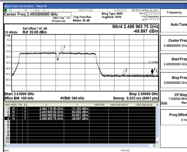
802.11n(HT40)-High channel
