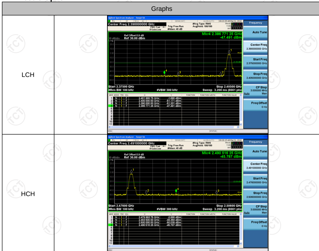
Test Graphs
