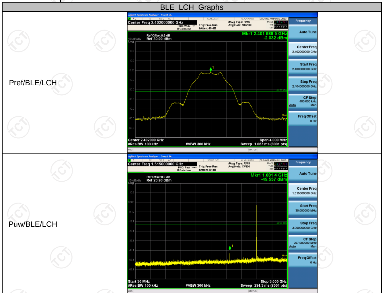
Test Graphs
