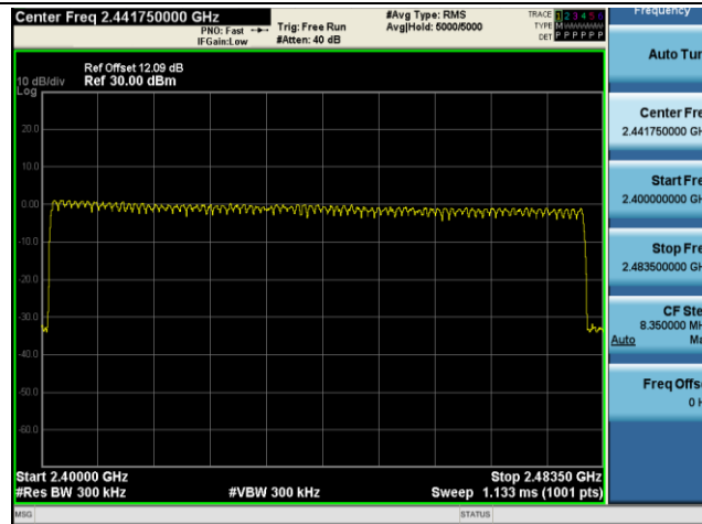
3DH5-Ant1-Hop
