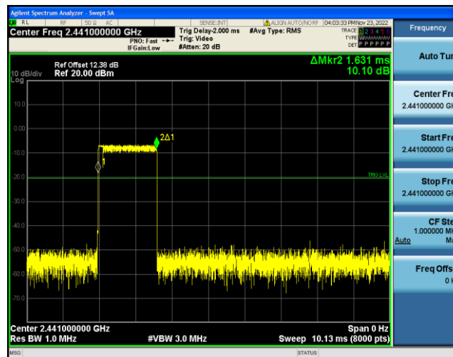
3DH5-Ant1-Hop-2.880-106.67
