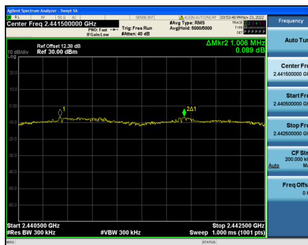
3DH5-Ant1-Hop
