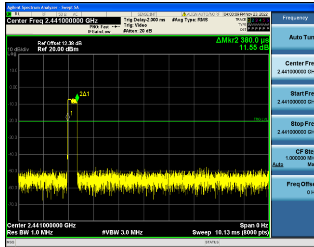
DH1-Ant1-Hop-0.371-320
