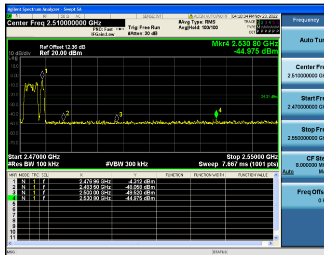
3DH5-Ant1-High-Hop_2480--4.31
