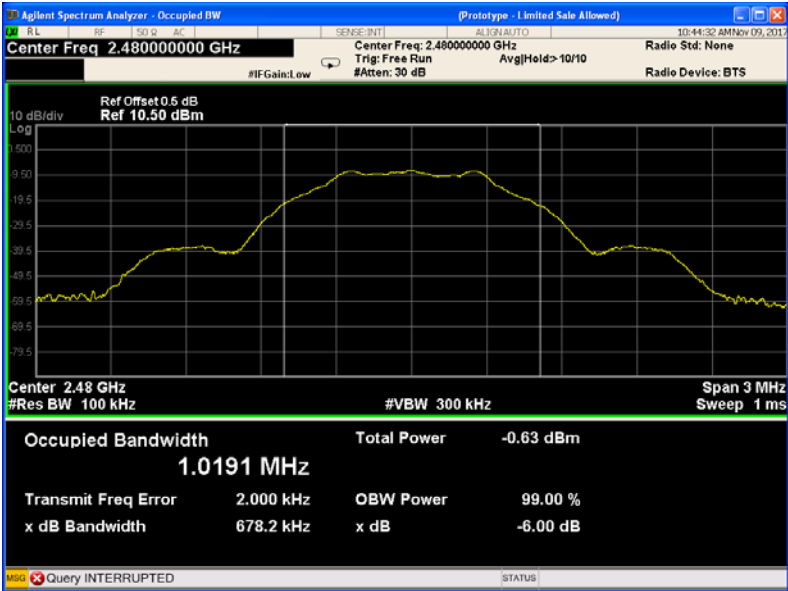
BLE: channel 39
