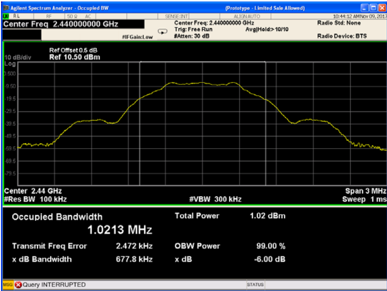
BLE: channel 19
