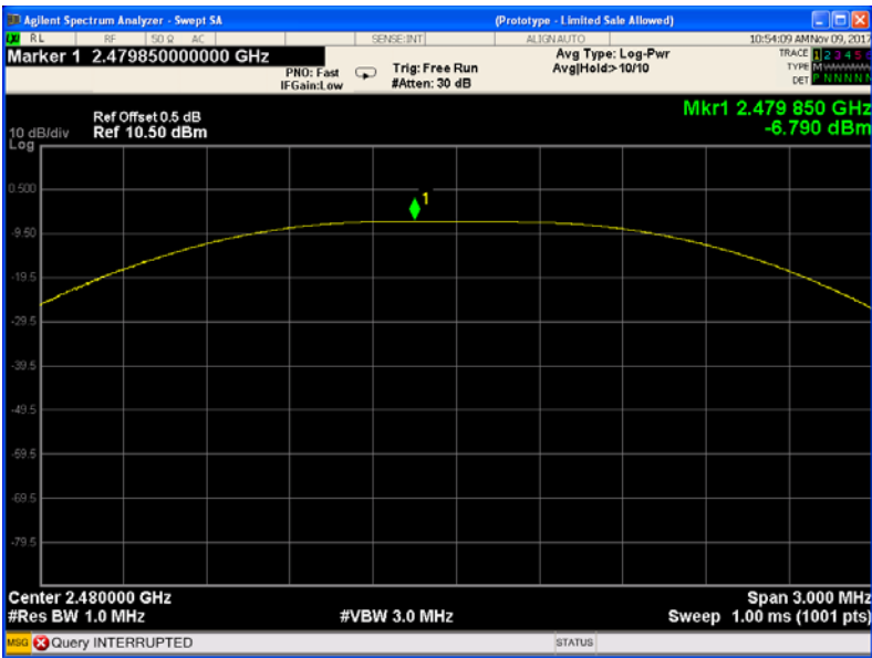
BLE: channel 39
