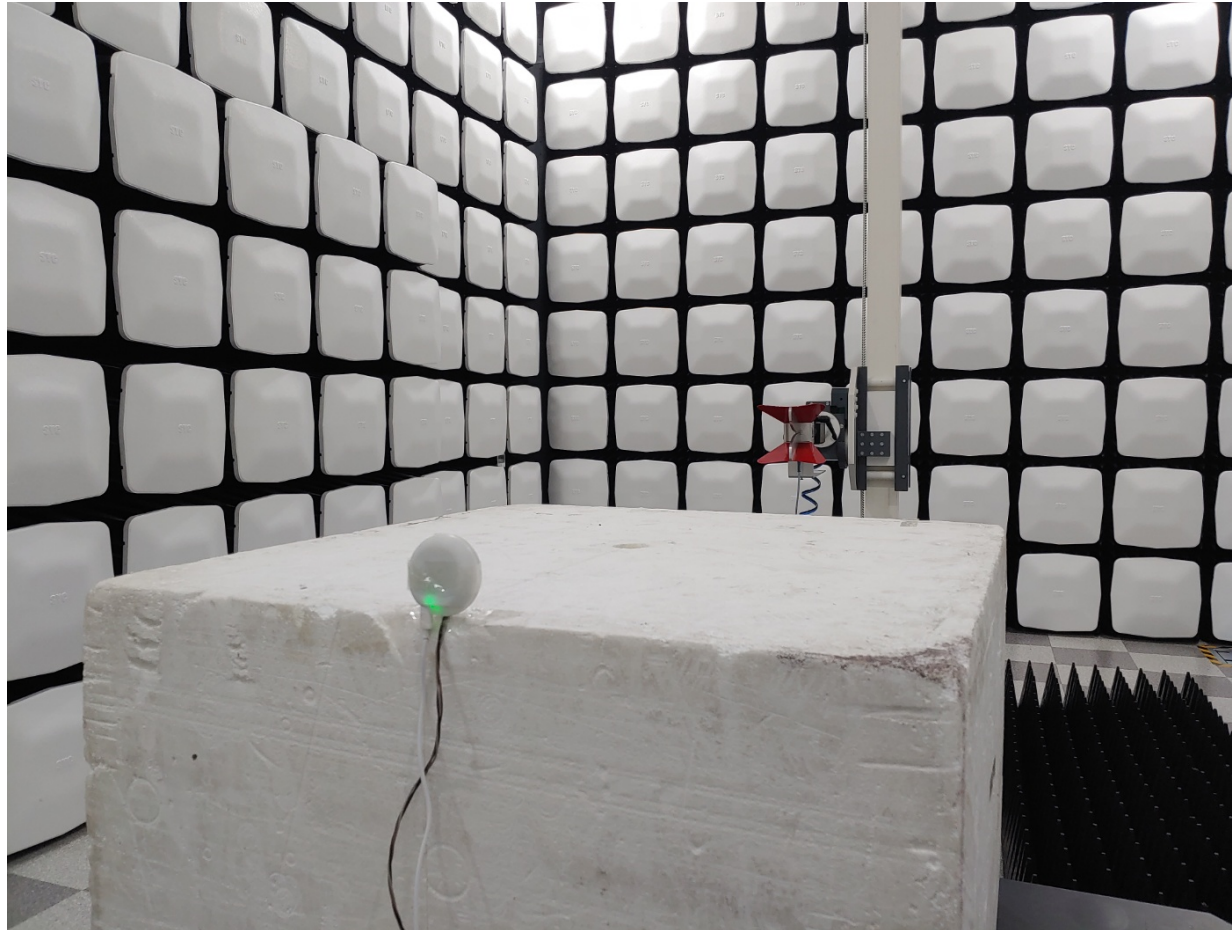
Radiated RF measurement (Above 1 GHz)_1m
