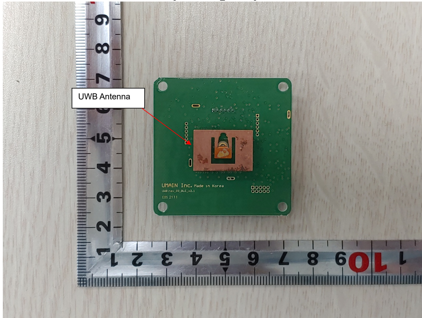
[Main board_Bottom]
