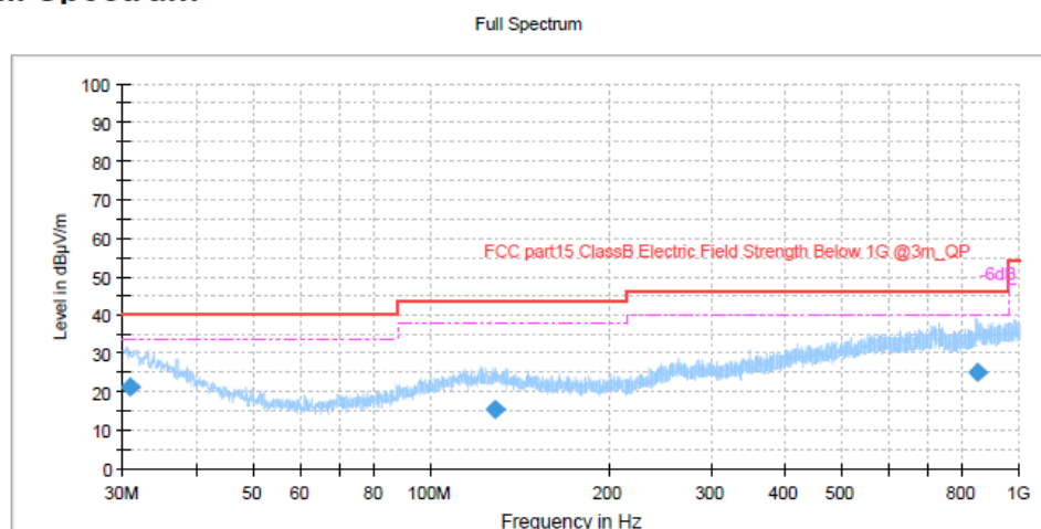
Figure 16: Spectral Diagrams, Radiated Emission, 30MHz-1000MHz, Vertical, 2DH5, 2480MHz
