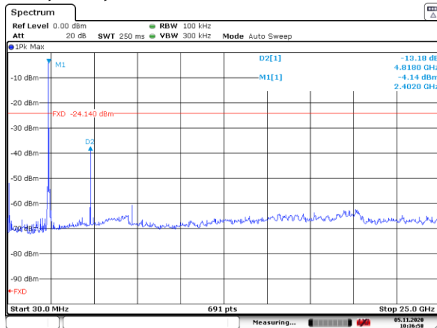
Figure 3: Conducted Spurious Emission
