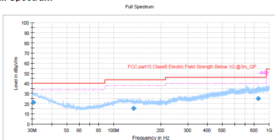
Figure 12: Spectral Diagrams, Radiated Emission, 30MHz-1000MHz, Vertical, DH5, 2480MHz
