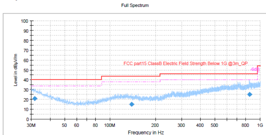
Figure 14: Spectral Diagrams, Radiated Emission, 30MHz-1000MHz, Vertical, 2DH5, 2402MHz
