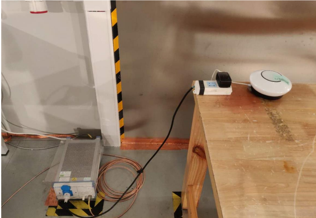
Set-up for Conducted Emission
