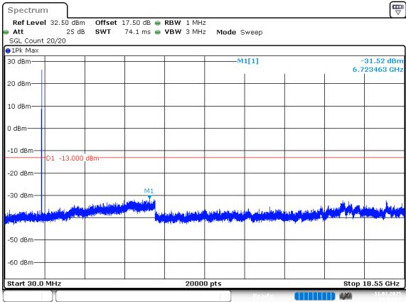
3MHz_Middle_QPSK_1@0(30MHz~18.55GHz)
