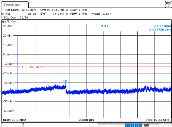
1.4MHz_High_QPSK_1@0(30MHz~18.55GHz)
