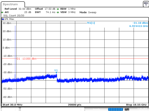
1.4MHz_Low_QPSK_1@0(30MHz~18.55GHz)
