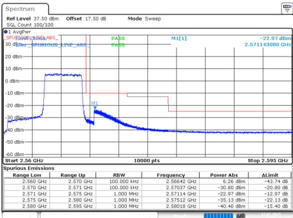
10MHz_High_16QAM_25@25
