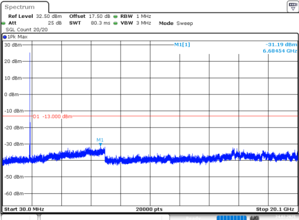
20MHz_High_QPSK_1@0(30MHz~20.1GHz)
