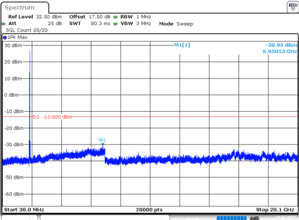
15MHz_Middle_QPSK_1@0(30MHz~20.1GHz)
