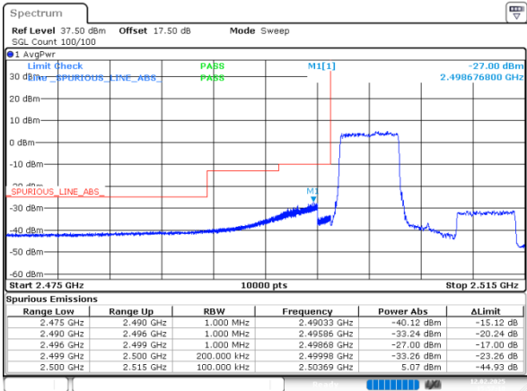
15MHz_Low_16QAM_25@0
