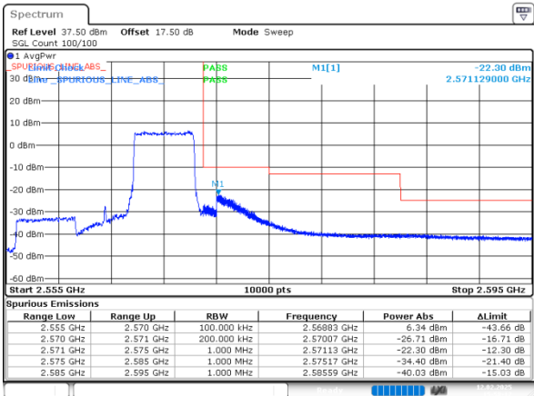
15MHz_High_16QAM_25@50
