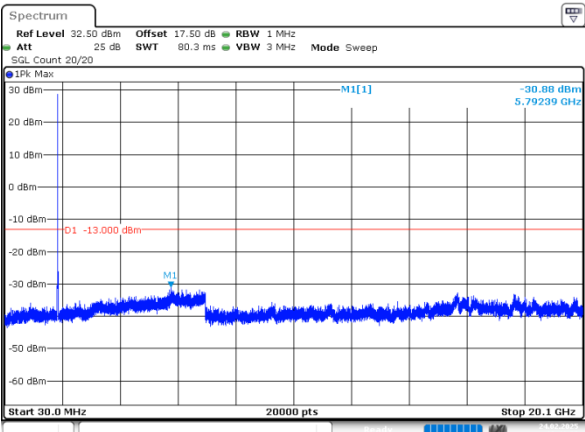
20MHz_Low_QPSK_1@0(30MHz~20.1GHz)
