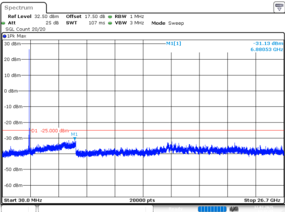
20MHz_High_QPSK_1@0(30MHz~26.7GHz)
