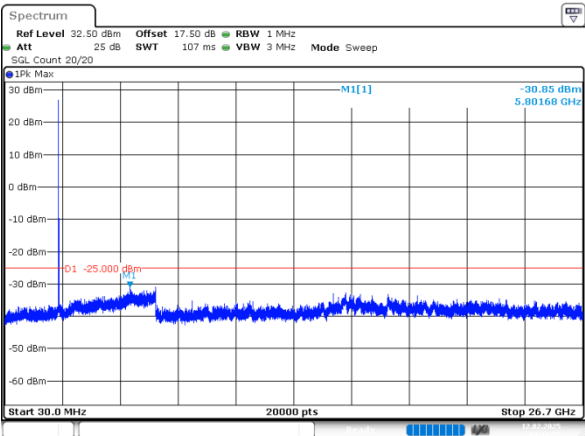
20MHz_Low_QPSK_1@0(30MHz~26.7GHz)
