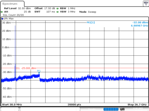
15MHz_Middle_QPSK_1@0(30MHz~26.7GHz)
