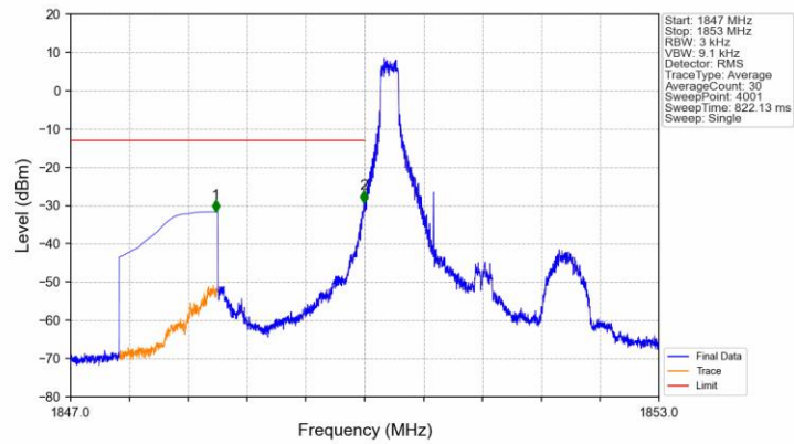
Band2_1.4MHz_QPSK_LCH_1850.7MHz_RB_1_0_NTNV
