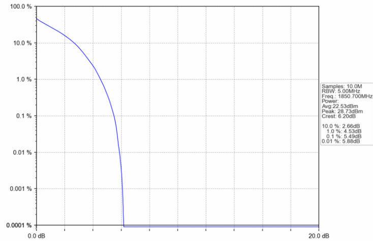
Band2_1.4MHz_QPSK_LCH_1850.7MHz_RB_6_0_NTNV
