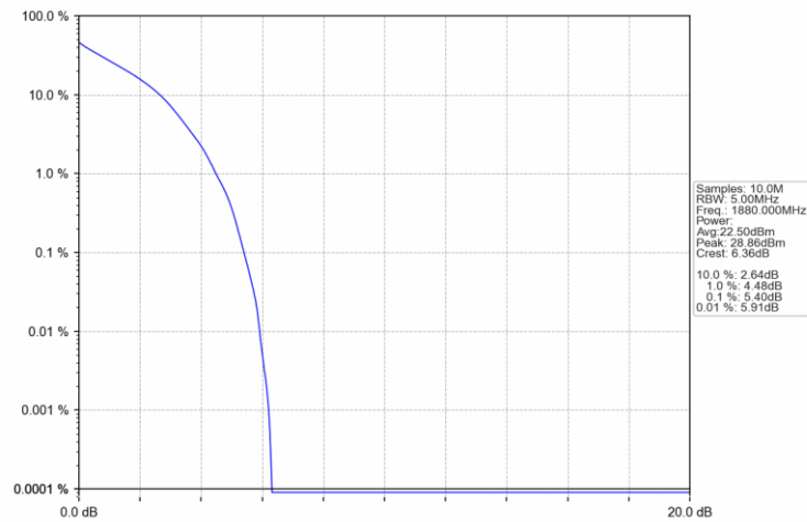
Band2_1.4MHz_QPSK_MCH_1880MHz_RB_6_0_NTNV
