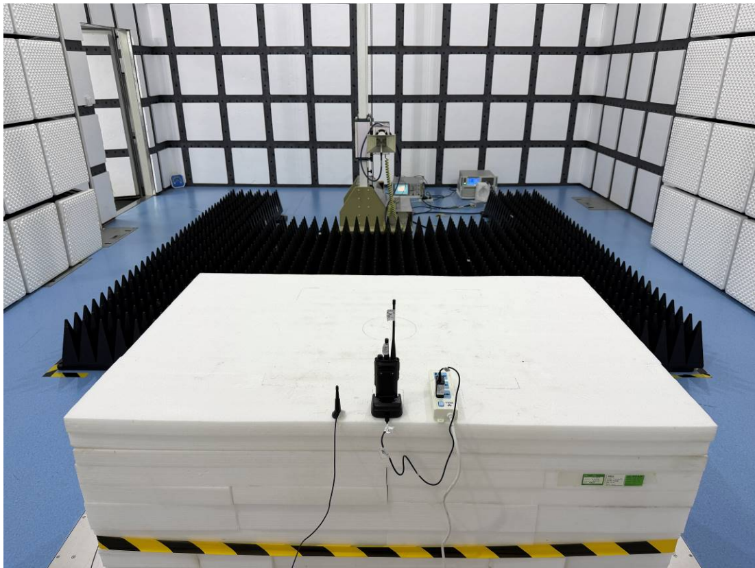
Radiation Emission - Back View (Above 1GHz) _Mode 2&4
