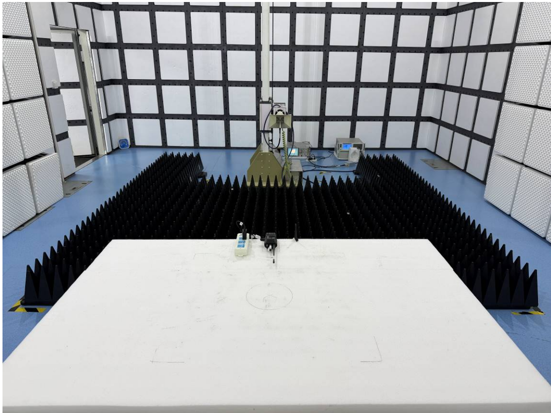
Radiation Emission - Back View (Above 1GHz) _Mode 1&3
