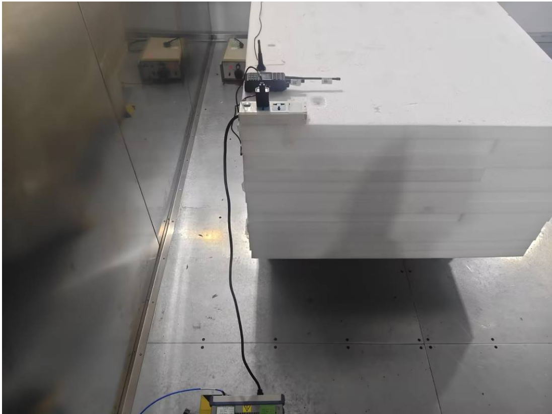
Conducted Emission - Side View _Mode 1&3
