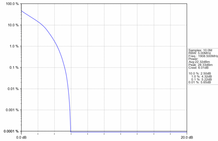
Band2 3MHz QPSK HCH 1908.5MHz RB 15 0 NTNV
