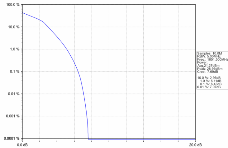
Band2 3MHz 16QAM LCH 1851.5MHz RB 15 0 NTNV
