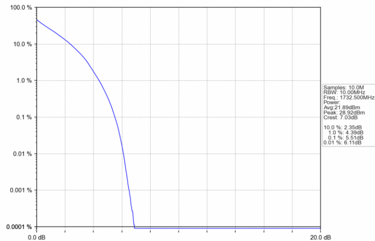
Band4_10MHz_QPSK_MCH_1732.5MHz_RB_50_0_NTNV
