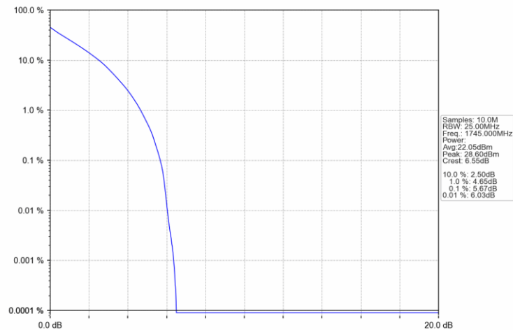
Band66_15MHz_QPSK_MCH_1745MHz_RB_75_0_NTNV
