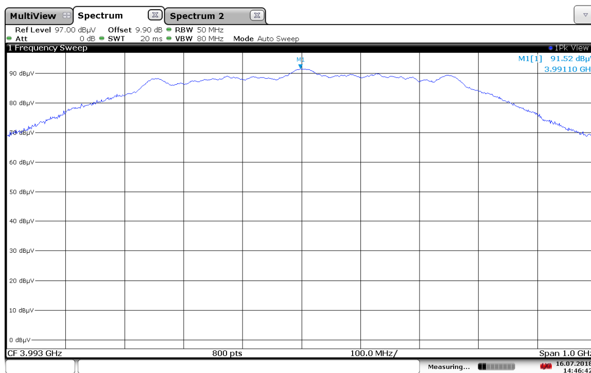
Figure 7.4.2-1: Peak Power Plot
