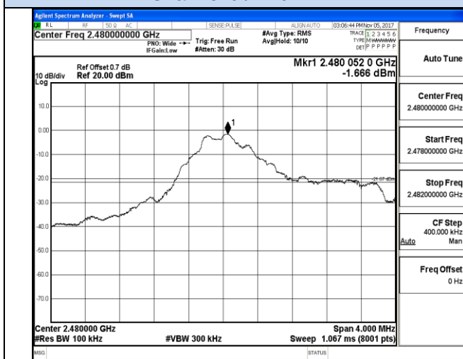
Channel 18 / 2480 MHz
