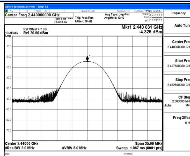
Channel 19 / 2440 MHz
