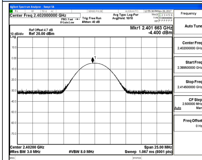
Channel 0 / 2402 MHz
