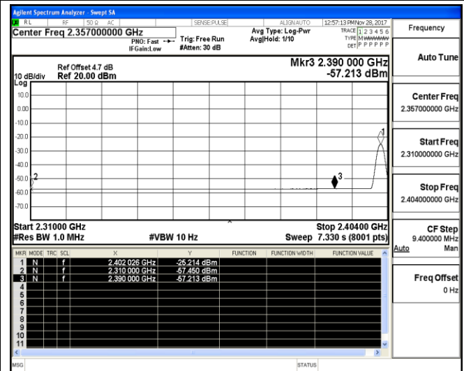
Channel 0 / 2402 MHz – Average
