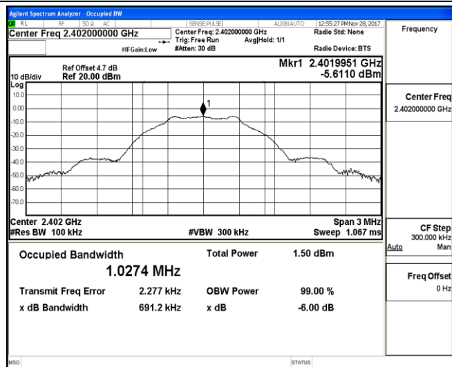
Channel 0 / 2402 MHz
