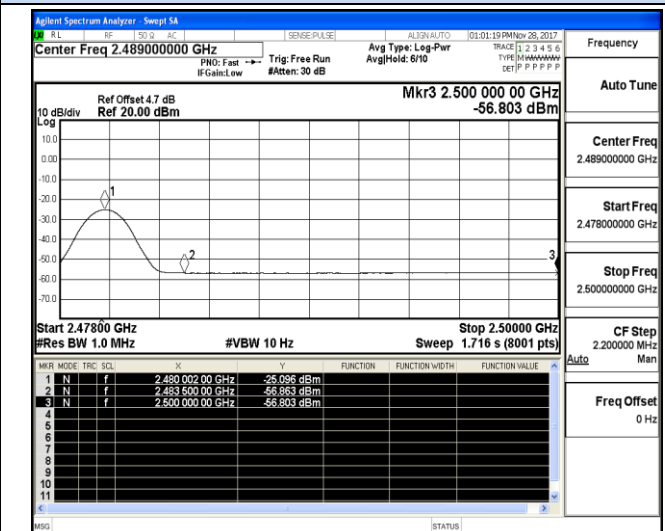
Channel 39 / 2480 MHz – Average
