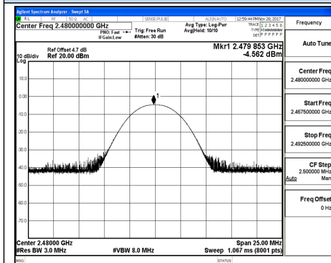
Channel 39 / 2480 MHz
