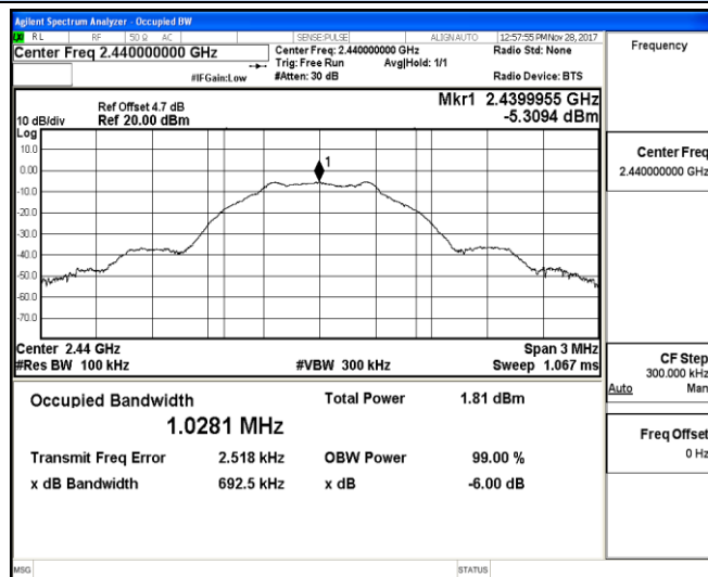
Channel 19 / 2440 MHz
