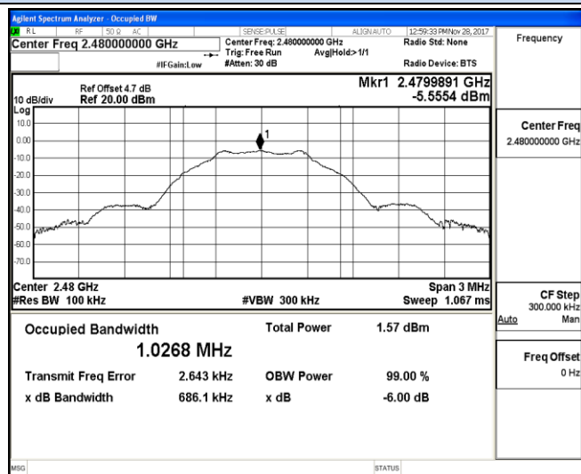
Channel 39 / 2480 MHz
