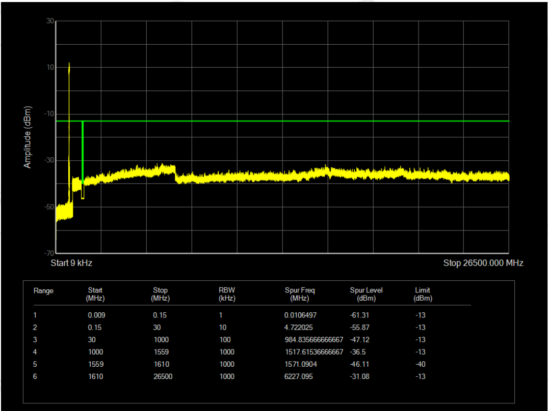
Band14 QPSK BW=10MHz Channel=23330 RB Size=50 Position=#0
