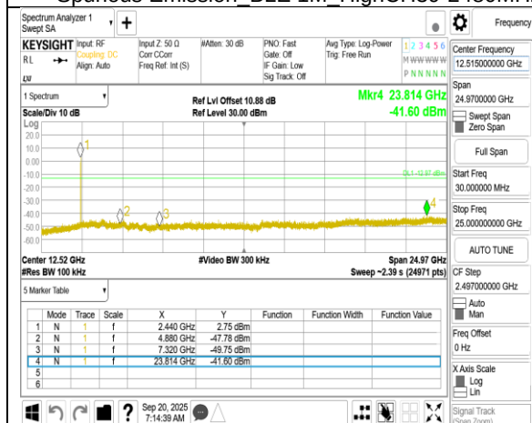
Spurious Emission_BLE 2M_MidCH19-2440MHz
