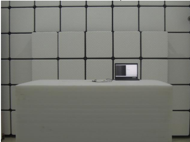
BT_Radiated_Setup
