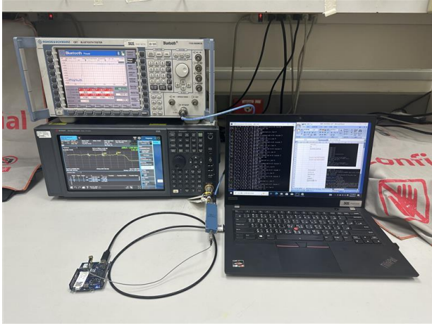
WLAN 2.4G_Conducted_Setup
