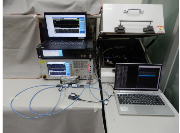
WLAN 5G_Normal_DFS_Slave_Setup
