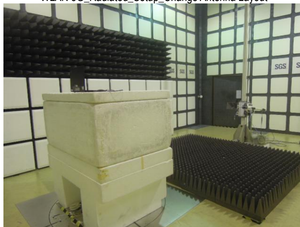
WLAN 5G_Radiated_Setup_Change Antenna Layout
