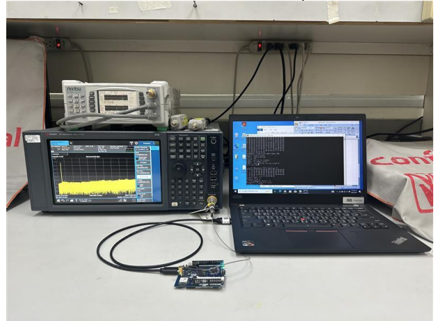
BLE_Radiated_Setup_Change Antenna Layout
