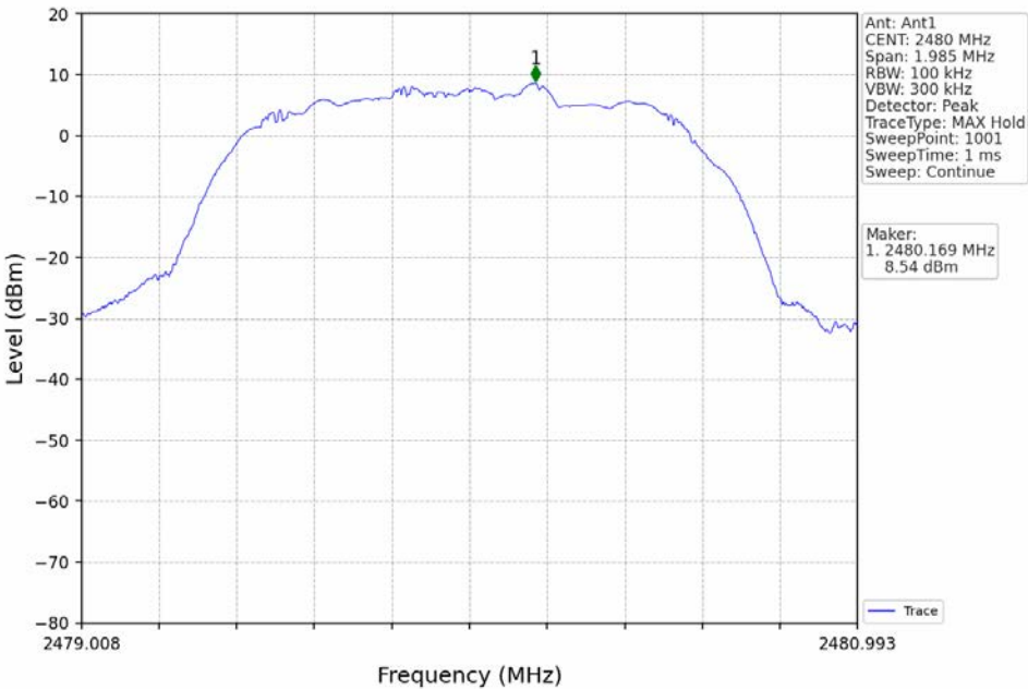
8DPSK_3DH5_HCH_2480MHz_Ant1_NTNV
