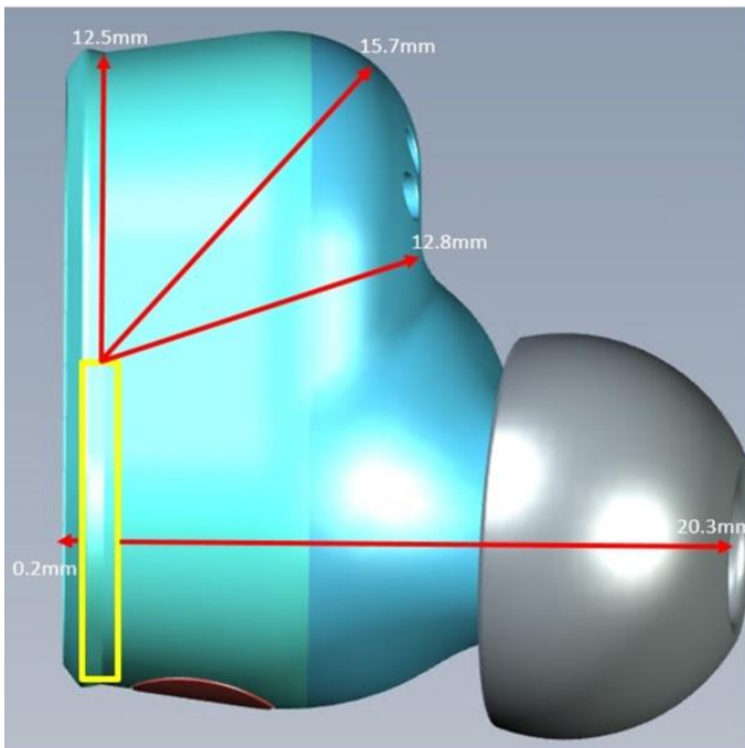
Right Earbud
